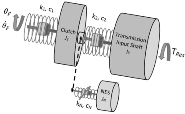
Fig. 5. Schematic representation of drivetrain equipped with a single NES.
