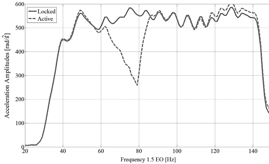
Fig. 10. Acceleration amplitude contribution at 1.5 EO at the transmission input shaft 1st gear engaged at 25% throttle) for a drivetrain equipped with a single NES ( J_N = 8\% of the transmission input shaft inertia, k_N = 1 \times 10^4 \text{ Nm/rad}^3 , c_N = 0.001 \text{ Nms/rad} ).
