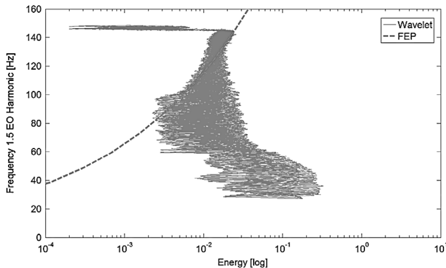
Fig. 18. FEP of the single NES exhibiting high AEAR with superposition of the 1.5 EO wavelet, targeting a high frequency range (1st gear engaged at 25% throttle).
