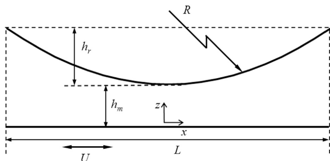
Fig. 9. Schematic of a converging-diverging symmetric parabolic contact profile.
