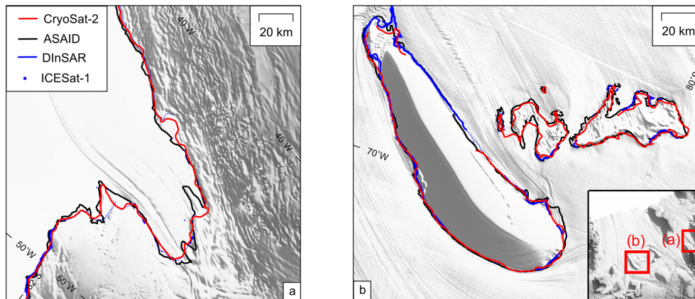
Figure 5. Grounding line mapped using DInSAR from both the MEaSUREs and the ESA CCI grounding line and ICESat-1 (blue), break in slope from the ASAlD project grounding line (Bindschadler et al., 2011) (black) and CryoSat-2 (red) methods for (a) Support Force Glacier and (b) Doake Ice Rumples. The background image is overlain on the REMA digital elevation model (DEM) (Howat et al., 2019).
