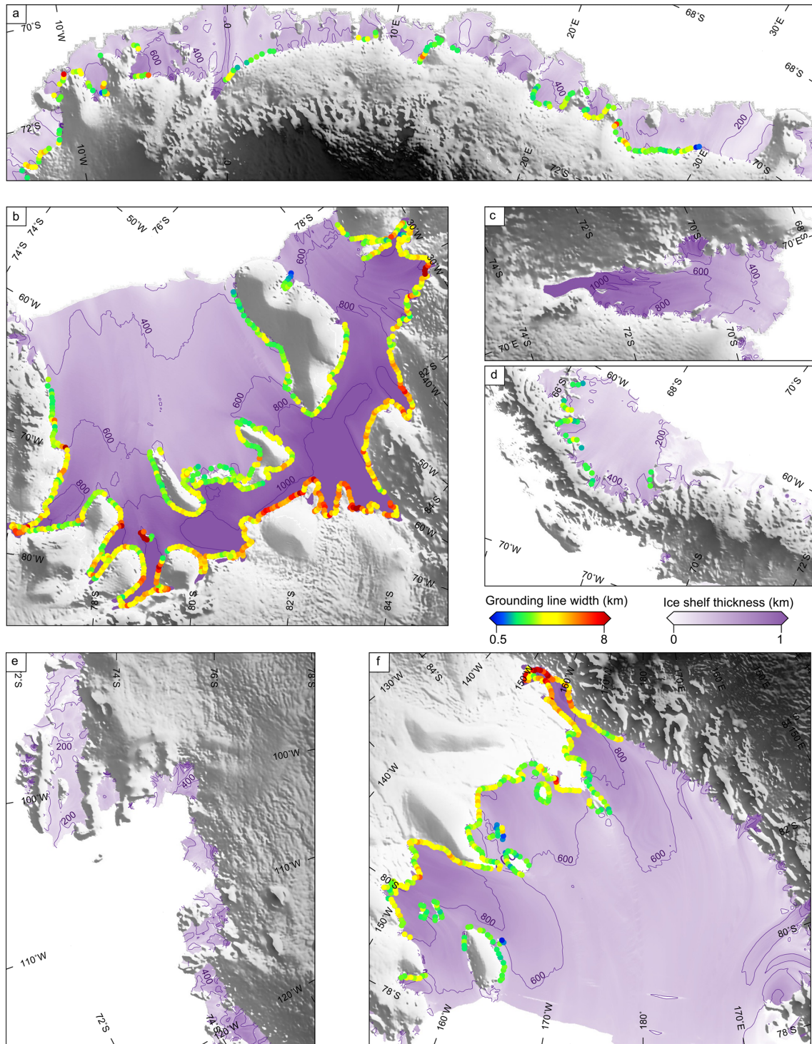
Figure 6. Grounding line width ( W ) for (a) Dronning Maud Land, (b) Filchner–Ronne Ice Shelf, (c) Amery Ice Shelf and (d) Antarctic Peninsula. (e) Amundsen Sea sector and (f) Ross Ice Shelf. The background image is the ice shelf thickness (Chuter and Bamber, 2015) overlain on the Bedmap-2 DEM (Fretwell et al., 2006).
