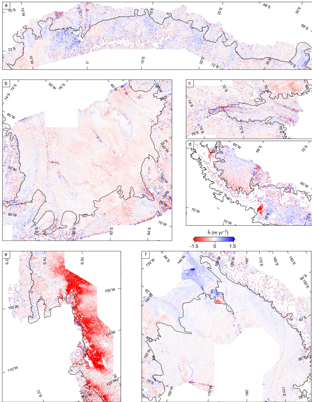
Figure A3. Elevation change ( h ) for (a) Dronning Maud Land, (b) Filchner–Ronne Ice Shelf, (c) Amery Ice Shelf and (d) Antarctic Peninsula. (e) Amundsen Sea sector and (f) Ross Ice Shelf.
