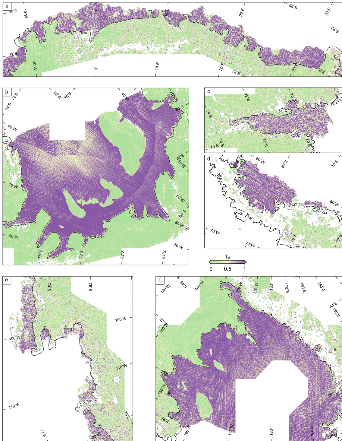
Figure 2. The dimensionless tidal amplitude, T_d , for (a) Dronning Maud Land, (b) Filchner–Ronne Ice Shelf, (c) Amery Ice Shelf and (d) Antarctic Peninsula. (e) Amundsen Sea sector and (f) Ross Ice Shelf. The black line is a composite grounding line by Depoorter et al. (2013).
