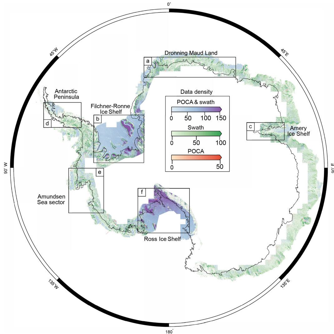
Figure 1. Data coverage plot for POCA (point of closest approach) and swath data. Red, green and blue data points correspond to where we used POCA, swath or both to calculate the tidal amplitude, T_d , respectively. The colour scales show the data density (POCA points per km). The swath data density is scaled by 150 (the average number of swath to POCA data points) to match the POCA density. The black line is a composite grounding line by Depoorter et al. (2013).
