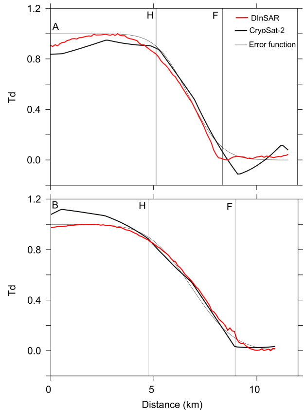
Figure 4. Cross sections of T_d (solid black line) with the fitted error function (dashed black line) and the normalised deformation measured from Sentinel-1 double-differenced interferograms (red line), for two cross sections across the Carlson Inlet (a) and Evans Ice Stream (b) as shown in Fig. 3.
