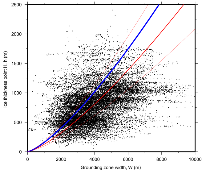
Figure 7. Grounding zone width ( W ) vs. ice thickness at point H ( h ). The solid red line is the fit of equation W = (26.4 \pm 6)h^{3/4} to the data, and the dashed red lines are the uncertainty bounds, while the blue line represents the estimation of Vaughan (1995) of W = (25.4 \pm 6.2)h^{3/4} .
