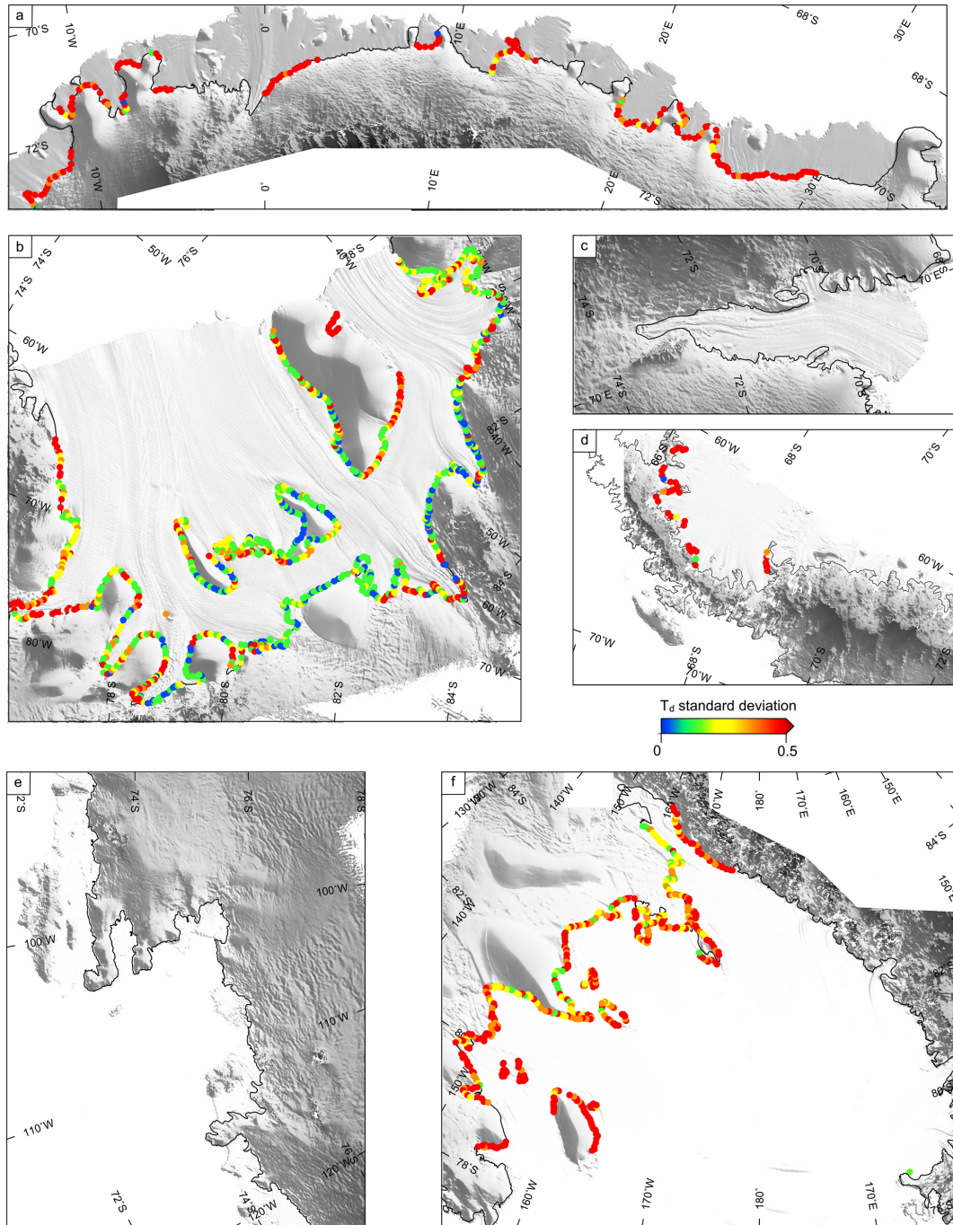
Figure A4. The standard deviation of T_d for the mapped grounding zone for (a) Dronning Maud Land, (b) Filchner-Ronne Ice Shelf, (c) Amery Ice Shelf and (d) Antarctic Peninsula. (e) Amundsen Sea sector and (f) Ross Ice Shelf.
