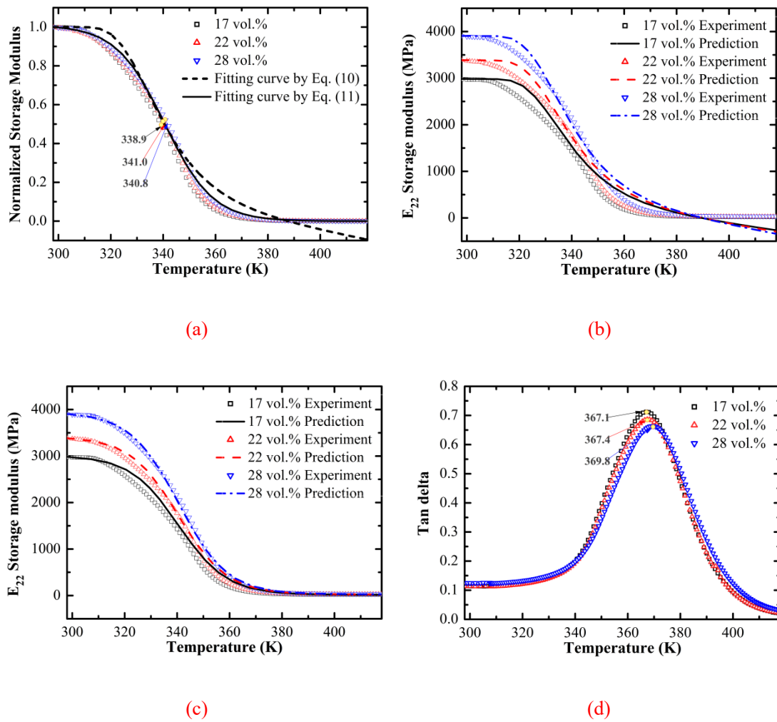
Fig. A.2. The DMA results of SMPCs with fiber direction perpendicular to the specimen's length, (a) normalized transverse storage moduli, (b) transverse storage moduli (prediction based on Eq. (10) ), (c) transverse storage moduli (prediction based on Eq. (11) ), (d) tan delta
