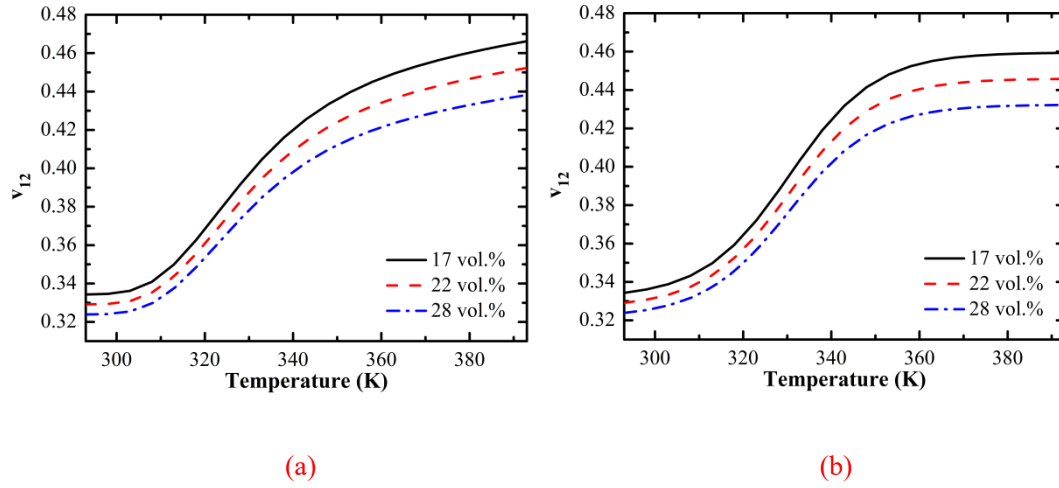
Fig. 6. Axial Poisson's ratios v_{12} of SMPCs at different temperatures, (a) results based on Eq. (10), (b) results based on Eq. (11)
