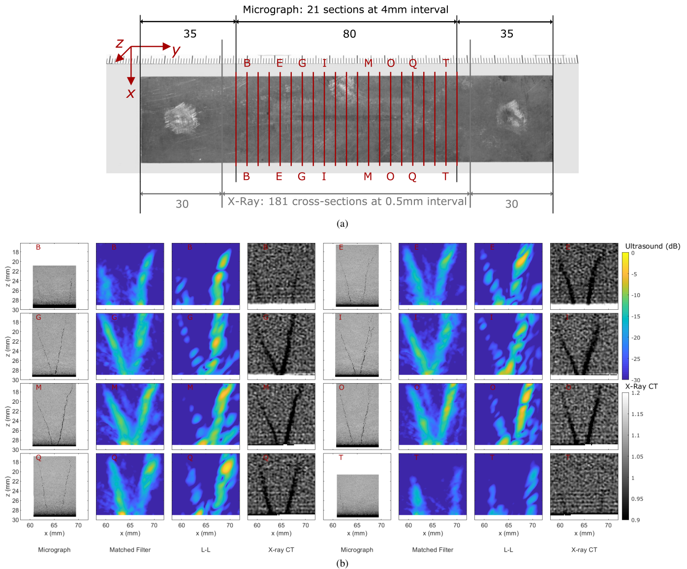
Fig. 7. Qualitative comparison between the matched filter fusion algorithm, the single L-L view and the X-ray CT and micrograph data at selected cross-sectional slices within Sample A. (a) Photo of the reduced Sample A, with relevant coverage of collaborating data overlaid. (b) Selected cross-section slices, with their locations indicated in (a).
