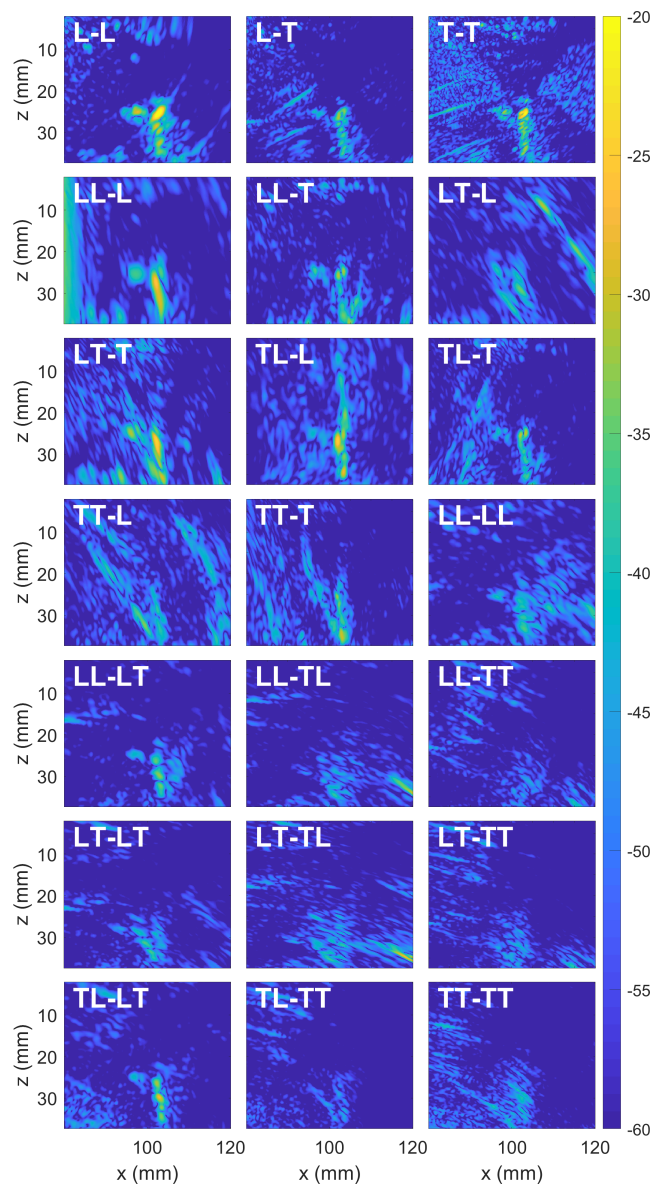
Fig. 11. Multi-view TFM images (in dB relative to the peak back wall response in the L-L view) of defect a (at y = 57\text{ mm} ) within Sample B.
