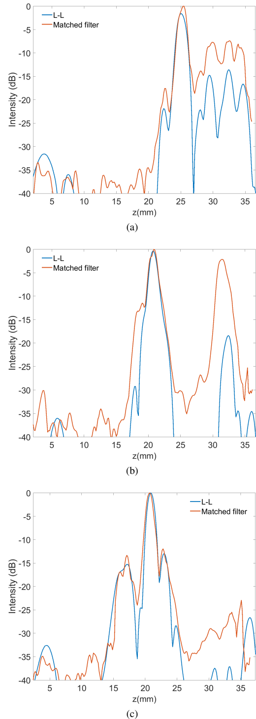
Fig. 13. Intensity profiles along defect vertical centreline in Sample B: (a) defect a ; (b) defect b ; (c) defect c . Each profile is normalised independently by its respective peak intensity.
