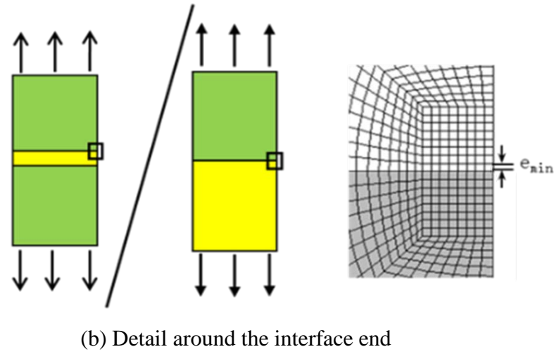
Fig.4 FEM mesh for the plate butt joint h/W=0.001 and simply bonded plate h/W=1
