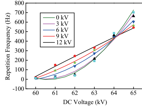
Fig. 5. Repetition frequency of current pulses.
