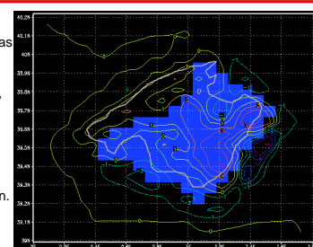
(Fig. 1b) Low-level convergence map over the Isle of Mallorca on July 27 th , 2004 (1115h UTC). The original grid-basis is bounded by 38°9'N and 40°22'N, and 2°00' and 3°83'E. Area coloured in blue corresponds to the set of 95 grid-points used for the linear correlation analysis
