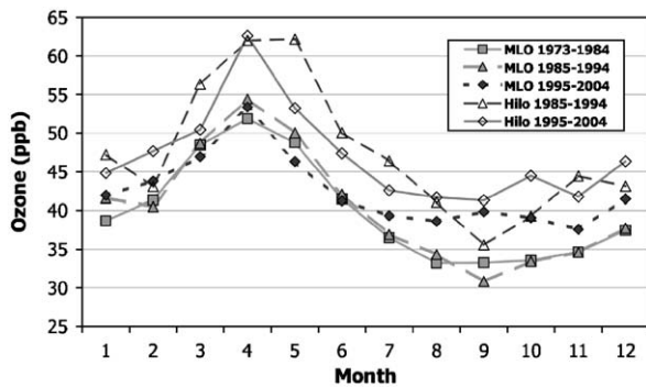
Fig. 13. Seasonal variation in surface ozone (filled symbols) at Mauna Loa Observatory (MLO) and in the 700–500 hPa layer ozone (open symbols) at Hilo, Hawaii, for different 10-year time periods.
