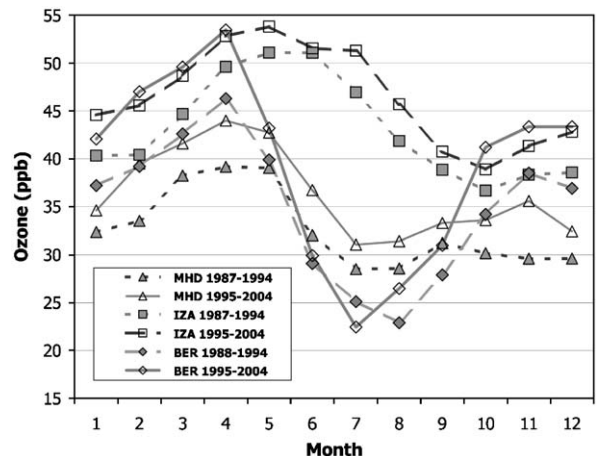
Fig. 7. Average monthly surface ozone for three sites in the North Atlantic for two time periods (MHD = Mace Head, IZA = Izaña, BER = Bermuda).
