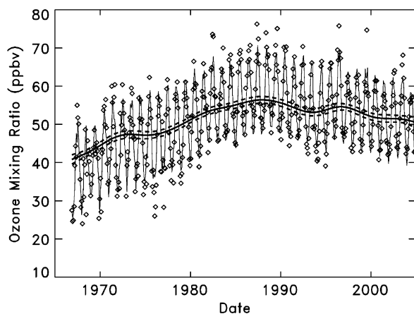
Fig. 5. Monthly average ozone amounts at Hohenpeissenberg in the 700–500 hPa layer (diamonds), the modeled values (gray solid line), and the fit (black solid curve) to the residuals (the difference between the data and the model) with the 95% confidence interval (black dashed curves).
