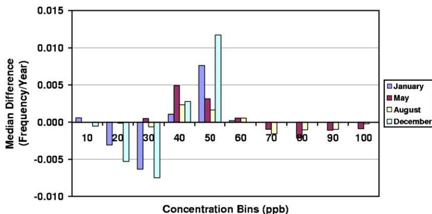
Fig. 12. The distribution of changes in surface ozone concentrations at Whiteface Mountain, New York, by month for months with significant changes in the distribution. The mass in the histogram for each month sums to one. The changes (pluses and minuses) add approximately to zero. A change in the frequency per year can be translated into hours by multiplying the plotted number by the total number of hours in the month. For example a month with 720 h and a frequency of 0.01 per year represents a shift from one concentration bin to another of 7 h per year. The median difference is computed by differencing between individual years (for example 1982–1983, 1982–1984, 1982–1985, ..., 1983–1984, 1983–1985, 1983–1986, ...). The plotted value is the median of these differences for each month and each concentration bin with a significant change.
