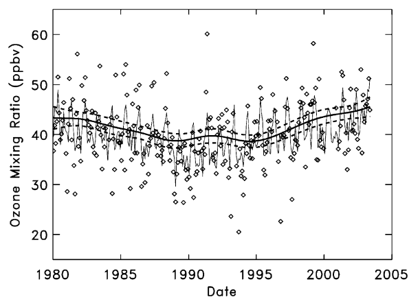
Fig. 3. Monthly average ozone amounts at Resolute in the 850–700 hPa layer (diamonds), the modeled values (gray solid line), and the fit (black solid curve) to the residuals (the difference between the data and the model) with the 95% confidence interval (black dashed curves).
