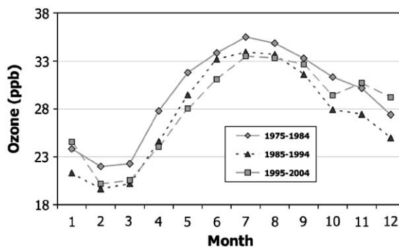
Fig. 21. Average monthly surface ozone at South Pole for three time periods.
