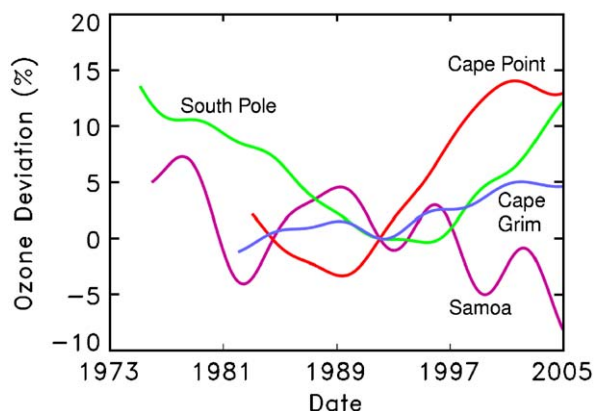
Fig. 16. Ozone trend curves (determined from the fit to the difference between the modeled data and the observations) in percent deviation at four selected S.H. surface ozone sites (South Pole—green, Cape Grim—blue, Cape Point—red, Samoa—magenta).
