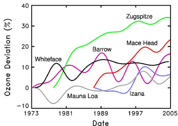
Fig. 1. Ozone trend curves (determined from the fit to the difference between the modeled data and the observations) in percent deviation at six selected N.H. surface ozone sites (Barrow—magenta, Mace Head—red, Zugspitze—green, Whiteface Mountain—black, Izana—blue, Mauna Loa—gray).
