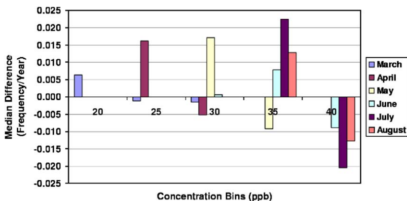
Fig. 22. The monthly change in the distribution of hourly average concentrations of South Pole surface ozone expressed as the median difference of occurrence of hourly averages in each concentration bin for each month with a significant change.
