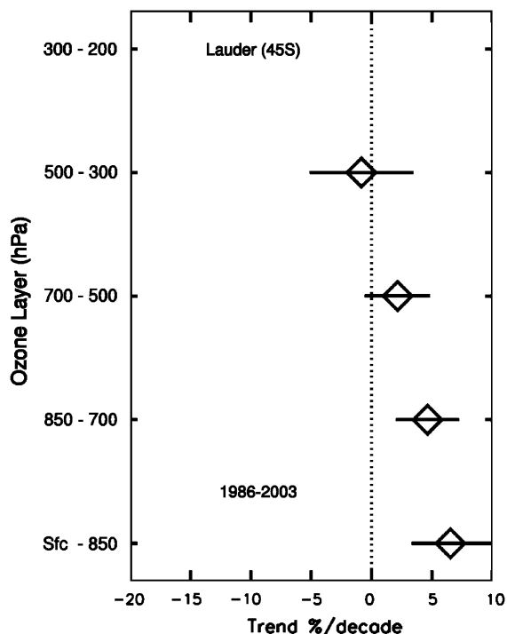
Fig. 19. Trend in altitude layers from ozonesonde data at Lauder, New Zealand.
