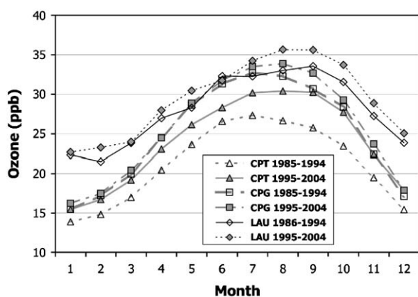
Fig. 18. Average seasonal cycle of surface ozone at Cape Point (CPT) and Cape Grim (CPG) and the 850–700 hPa layer average ozone at Lauder (LAU) for two time periods.
