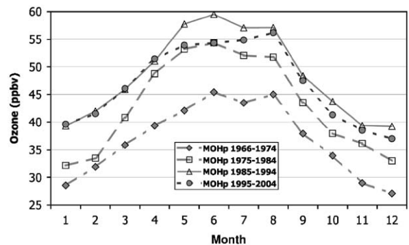
Fig. 6. Average monthly 850–700 hPa layer average ozone at Hohenpeissenberg for three time periods.
