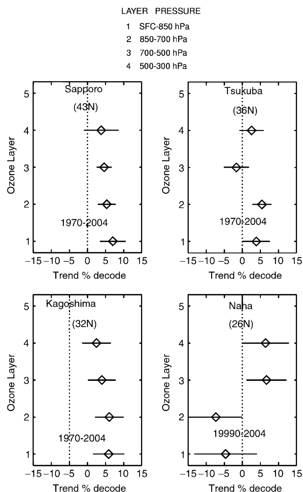
Fig. 9. Trend with altitude of the ozonesonde layer averages at four Japanese stations. Sapporo, Tsukuba and Kagoshima data are for the period 1970–2004 while Naha only includes the period 1990–2004.
