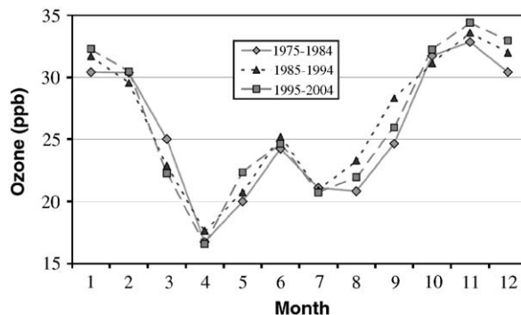
Fig. 2. Average monthly surface ozone at Barrow, Alaska, for three time periods.
