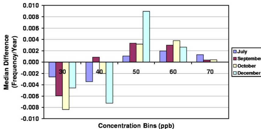
Fig. 14. The monthly change in the distribution of hourly average concentrations of Mauna Loa surface ozone expressed as the median difference of occurrence of hourly averages in each concentration bin for each month with a significant change.
