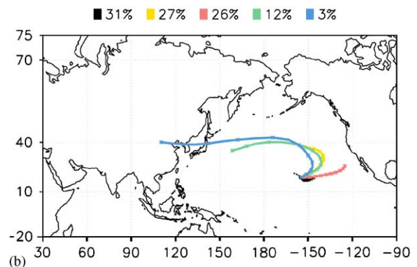
Fig. 15. Clustered trajectories for Mauna Loa Observatory for the months of September and October for the (a) 1986–1994 and (b) 1995–2004 time periods.
