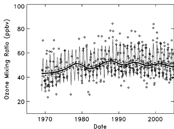
Fig. 8. Monthly average ozone amounts at Tsukuba in the 850–700 hPa layer (diamonds), the modeled values (gray solid line), and the fit (black solid curve) to the residuals (the difference between the data and the model) with the 95% confidence interval (black dashed curves).
