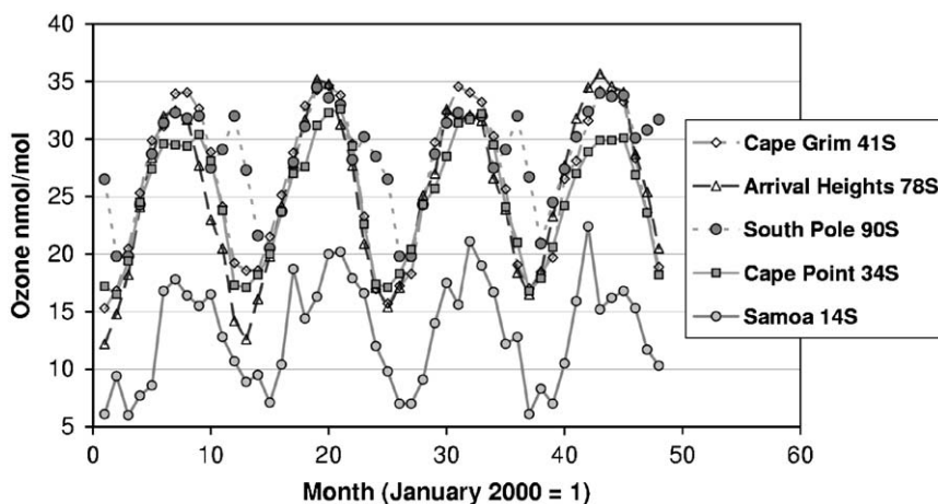
Fig. 17. Time series of monthly mean surface ozone at five sites in the S.H. for the period 2000–2003.
