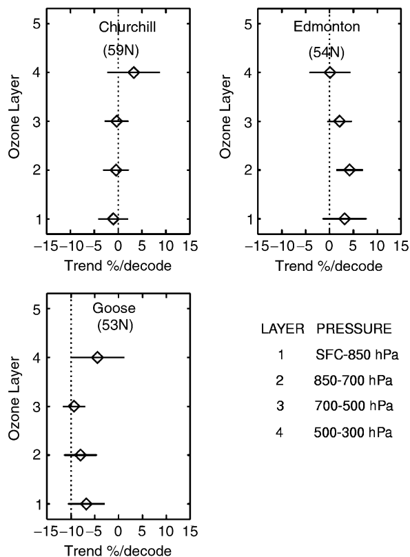
Fig. 10. Trend with altitude of the ozonesonde layer averages at three Canadian stations for the period 1980–2004.
