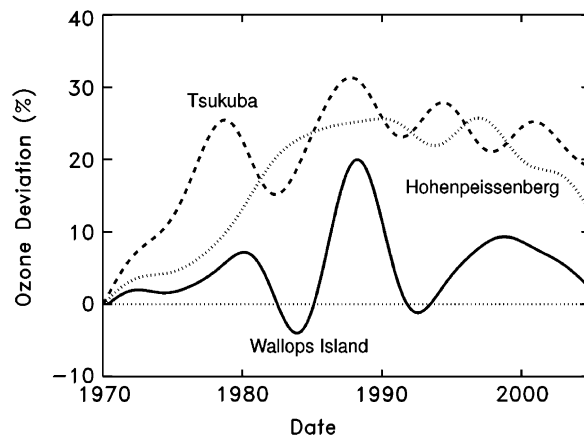
Fig. 11. Ozone trend curves (determined from the fit to the difference between the modeled data and the observations) in percent deviation for Hohenpeissenberg, Tsukuba, and Wallops Island for the 850–700 hPa layer.
