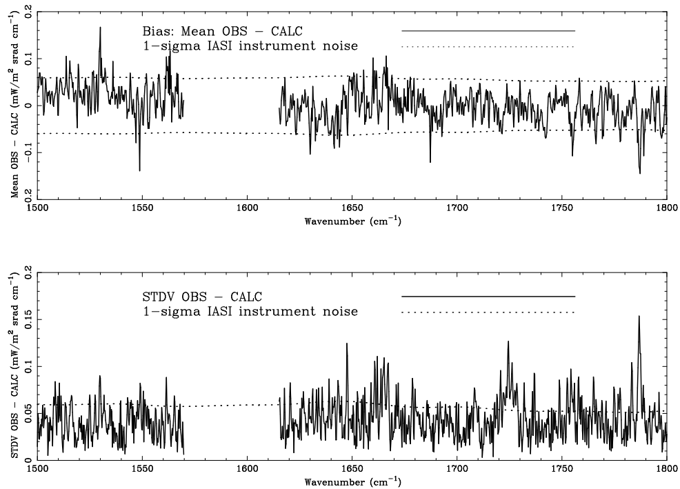
Fig. 14. Bias and standard deviation of IASI observed minus calculated radiances. The calculated radiances have been obtained using OSS and the “in situ” bias correction.
