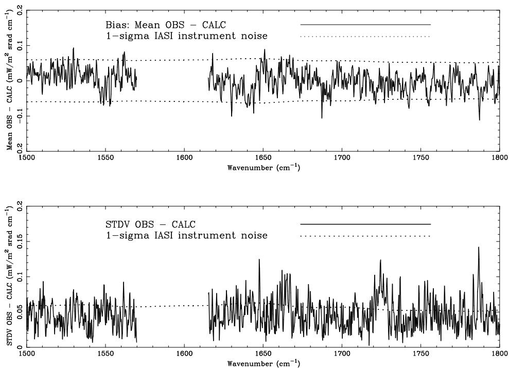
Fig. 15. Bias and standard deviation of IASI observed minus calculated radiances. The calculated radiances have been obtained using LBLRTM 11.6 and the “in situ” bias correction.
