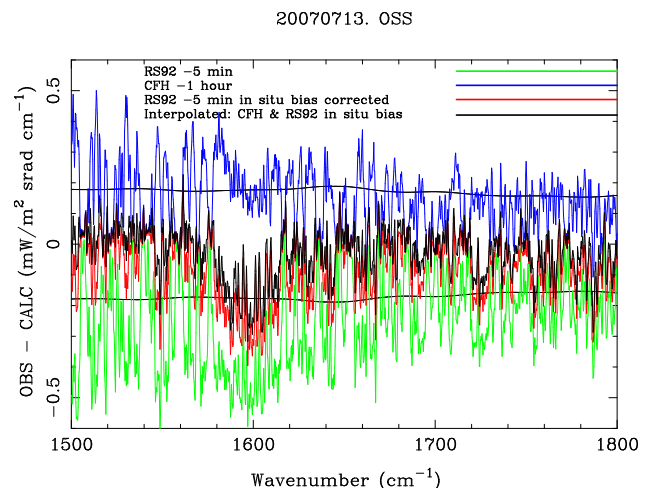
Fig. 6. Residual radiances, IASI observed minus calculated with OSS RTM, for different atmospheric profiles: CFH sonde launched 1 h before overpass (blue), RS92 sonde launched 5 min before overpass (green), same sonde but with the “in situ” bias correction (red) and the time interpolated profile (black) using CFH (launched 1 h before overpass) and “in situ” bias corrected RS92 (launched 5 min before overpass) measurements. Thin black nearly flat lines correspond to three sigma IASI instrument noise.
