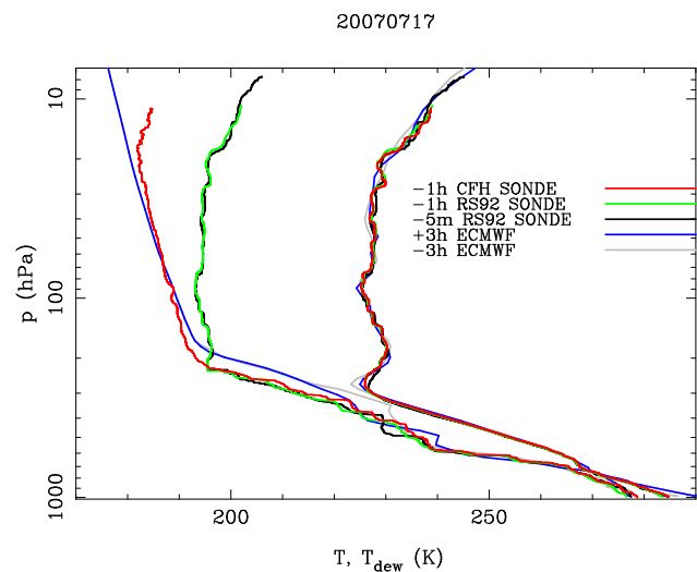
Fig. 5. Temperature (right) and water vapour profiles (left) for the CFH and RS92 sonde launched 1 h before overpass time (red and green, respectively), the RS92 sonde launched 5 min before IASI overpass (black) and the ECMWF analysis profile approximately 3 h before and after satellite overpass (grey and blue, respectively). Note the big difference between the ECMWF analyses and the radiosondes moisture at 200 hPa.
