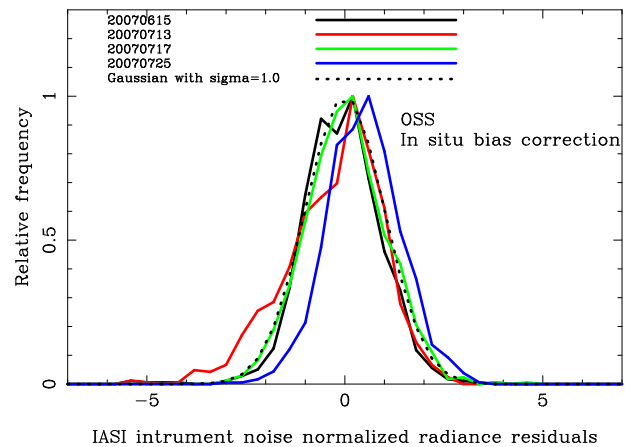
Fig. 13. Histogram of the residual radiances, IASI observed minus calculated with OSS RTM and the time interpolated profiles, for all clear days (4) in the spectral range, 1500 \text{ cm}^{-1} \leq \nu \leq 1570 \text{ cm}^{-1} and 1615 \text{ cm}^{-1} \leq \nu \leq 1800 \text{ cm}^{-1} . The interpolated profile has been derived from the CFH sonde launched 1 h before IASI overpass and the “in situ” bias corrected RS92 sonde launched 5 min before satellite overpass. The results for each one of the different observing days are shown independently in this figure. A one sigma Gaussian is shown as a dotted line.
