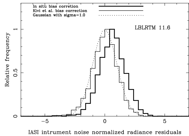
Fig. 11. Histogram of the residual radiances, IASI observed minus calculated with LBLRTM 11.6 RTM and time interpolated profiles, for all clear days (4) in the spectral range, 1500 \text{ cm}^{-1} \leq \nu \leq 1570 \text{ cm}^{-1} and 1615 \text{ cm}^{-1} \leq \nu \leq 1800 \text{ cm}^{-1} . One set of interpolated profile have been derived from the CFH sonde launched 1 h before IASI overpass and the “in situ” bias corrected RS92 sonde launched 5 min before satellite overpass (thick solid line). The other set of interpolated profiles have been derived from the CFH sonde launched 1 h before IASI overpass and the Kivi et al. bias corrected RS92 sonde launched 5 min before satellite overpass (thin solid line). For reference, a Gaussian curve with a \sigma of 1.0 is shown (dotted line).
