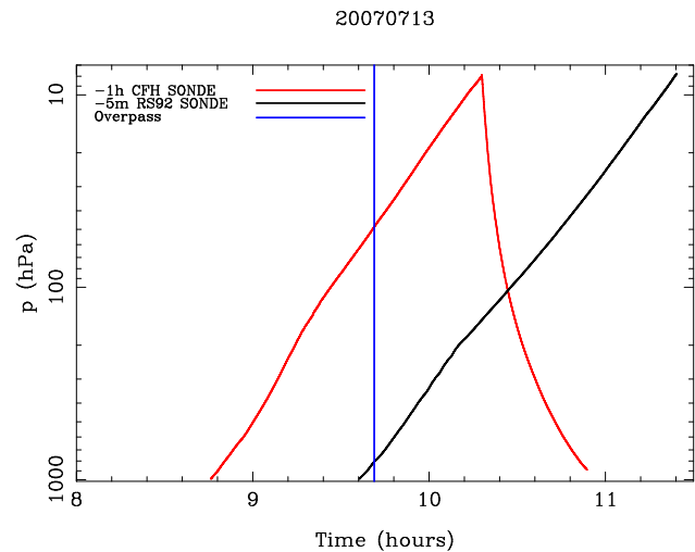
Fig. 3. Vertical position of the sonde versus time. The sonde, which carries an RS92 and a CFH, launched 1 h before overpass time is plotted (red) together with the sonde, carrying only an RS92, launched 5 min before overpass time (black). The overpass time is plotted as a vertical line (blue).
