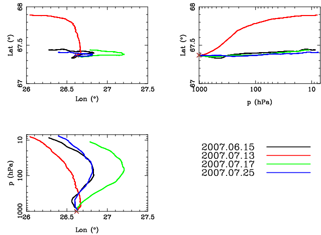
Fig. 2. Ascending trajectories of the four CFH sondes selected for comparison as shown in Table 1. The big brown cross is the launch location at the FMI Arctic Research Centre observatory in Sodankylä.
