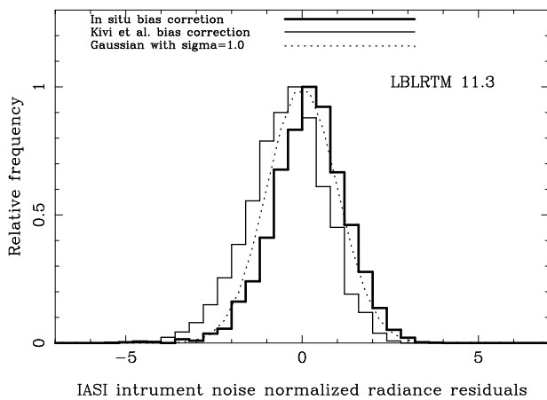
Fig. 10. Histogram of the residual radiances, IASI observed minus calculated with LBLRTM 11.3 RTM and time interpolated profiles, for all clear days (4) in the spectral range, 1500 \text{ cm}^{-1} \leq \nu \leq 1570 \text{ cm}^{-1} and 1615 \text{ cm}^{-1} \leq \nu \leq 1800 \text{ cm}^{-1} . One set of interpolated profiles have been derived from the CFH sonde launched 1 h before IASI overpass and the “in situ” bias corrected RS92 sonde launched 5 min before satellite overpass (thick solid line). The other set of interpolated profiles have been derived from the CFH sonde launched 1 h before IASI overpass and the Kivi et al. bias corrected RS92 sonde launched 5 min before satellite overpass (thin solid line). For reference, a Gaussian curve with a \sigma of 1.0 is shown (dotted line).
