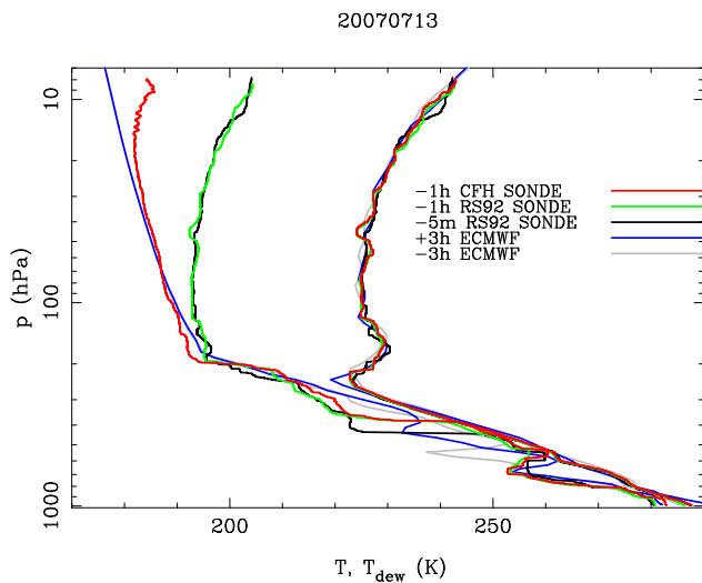
Fig. 4. Temperature (right) and water vapour profiles (left) for the CFH and RS92 sonde launched 1 h before overpass time (red and green, respectively), the RS92 sonde launched 5 min before IASI overpass (black) and the ECMWF analysis profile approximately 3 h before and after satellite overpass (grey and blue, respectively). Note the big moisture variation between the 1 h and 5 min before overpass launch measurements at the 400 hPa-level.
