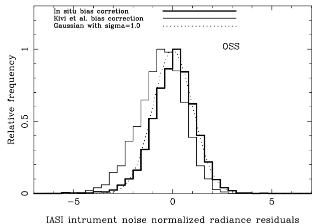
Fig. 9. Histogram of the residual radiances, IASI observed minus calculated with OSS RTM and time interpolated profiles, for all clear days (4) in the spectral range, 1500 \text{ cm}^{-1} \leq \nu \leq 1570 \text{ cm}^{-1} and 1615 \text{ cm}^{-1} \leq \nu \leq 1800 \text{ cm}^{-1} . One set of interpolated profiles have been derived from the CFH sonde launched 1 h before IASI overpass and the “in situ” bias corrected RS92 sonde launched 5 min before satellite overpass (thick solid line). The other set of interpolated profiles have been derived from the CFH sonde launched 1 h before IASI overpass and the Kivi et al. bias corrected RS92 sonde launched 5 min before satellite overpass (thin solid line). For reference, a Gaussian curve with a \sigma of 1.0 is shown (dotted line).
