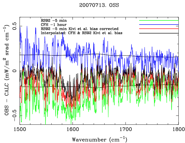
Fig. 7. Residual radiances, IASI observed minus calculated with OSS RTM, for different atmospheric profiles: CFH sonde launched 1 h before overpass (blue), RS92 sonde launched 5 min before overpass (green), same sonde but with the Kivi et al. bias correction (red) and the time interpolated profile (black) using CFH (launched 1 h before overpass) and Kivi et al. bias corrected RS92 (launched 5 min before overpass) measurements. Thin black nearly flat lines correspond to three sigma IASI instrument noise.
