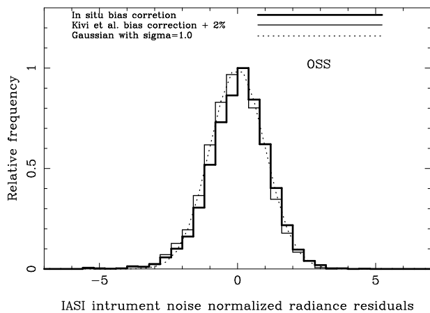
Fig. 12. Histogram of the residual radiances, IASI observed minus calculated with OSS RTM and time interpolated profiles, for all clear days (4) in the spectral range, 1500 \text{ cm}^{-1} \leq \nu \leq 1570 \text{ cm}^{-1} and 1615 \text{ cm}^{-1} \leq \nu \leq 1800 \text{ cm}^{-1} . One set of interpolated profiles have been derived from the CFH sonde launched 1 h before IASI overpass and the “in situ” bias corrected RS92 sonde launched 5 min before satellite overpass (thick solid line). The other set of interpolated profiles have been derived from the CFH sonde launched 1 h before IASI overpass and the Kivi et al. +2% bias corrected RS92 sonde launched 5 min before satellite overpass (thin solid line). For reference, a Gaussian curve with a \sigma of 1.0 is shown (dotted line).
