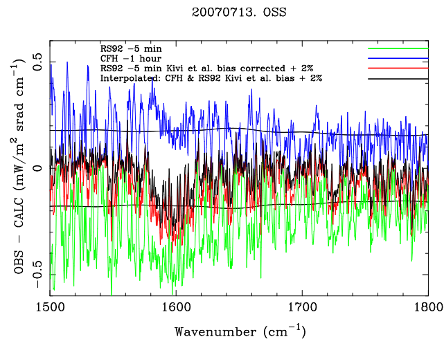
Fig. 8. Residual radiances, IASI observed minus calculated with OSS RTM, for different atmospheric profiles: CFH sonde launched 1 h before overpass (blue), RS92 sonde launched 5 min before overpass (green), same sonde but with the “Kivi et al. +2” bias correction (red) and the time interpolated profile (black) using CFH (launched 1 h before overpass) and Kivi et al. +2 bias corrected RS92 (launched 5 min before overpass) measurements. Thin black nearly flat lines correspond to three sigma IASI instrument noise.
