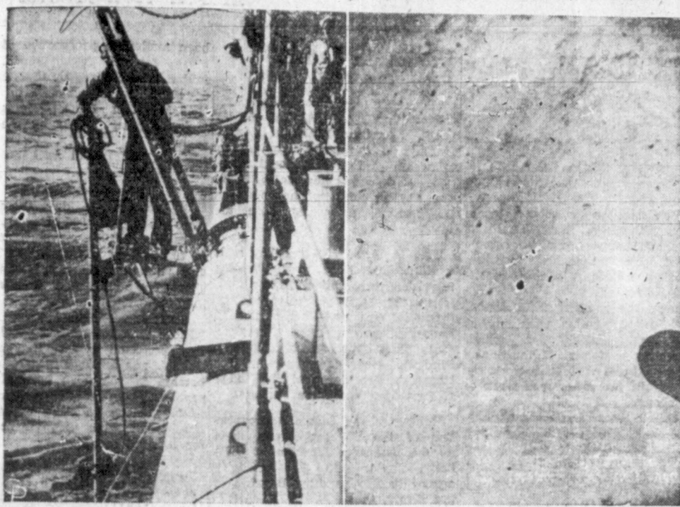
PHOTOGRAPHIC EQUIPMENT is lowered (left) from the U. S. Navy oceanographic ship San Pablo in the Sargasso sea, a part of the Atlantic some 1,000 miles from Cape Hatteras, N. C. Here (right) is what the camera caught at 20,800 feet, greatest depth the ocean ever has been photographed. It is a somewhat blank sea bottom, pocked by holes made by marine creatures. Dark object at right is part of light source used for making the picture. A 14-foot camera of aluminum in shape of a pipe was used for the
