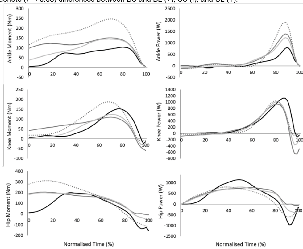
Figure 2. Joint moment- (left) and power- (right) normalised time curves for the front ankle (top), knee (middle) and hip (bottom) joint during BS (black), BL (dark grey), SS (light grey) and UL (dotted).
