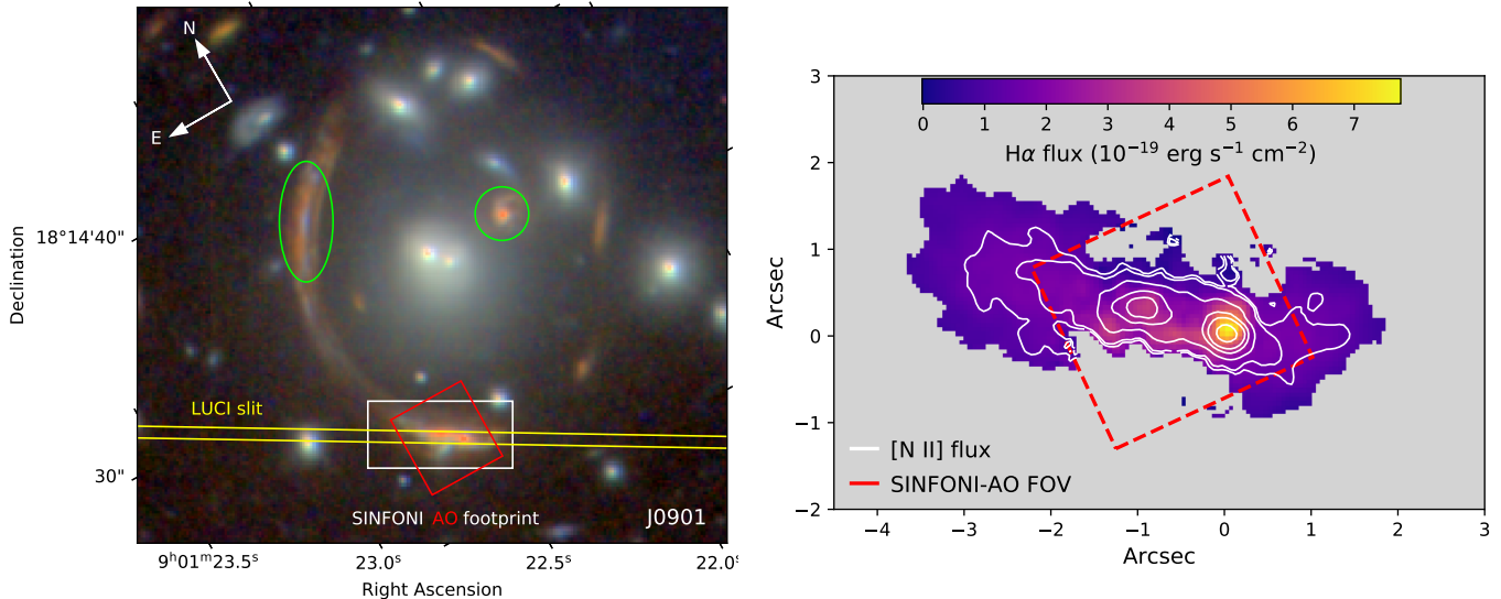
Figure 4. Left: J0901 color composite using HST F160W (red) + F110W (green) + F814W (blue), with the footprints of the LUCI slit (yellow), and the SINFONI seeing limited (white) and AO (red) data overplotted. J0901 is triply imaged by the lensing cluster. The south eastern image is at the center of the SINFONI footprint, and the north eastern and western images are indicated by the green ellipses. Right: Image plane H \alpha flux map of J0901, constructed by combining the AO data (inside the red rectangle) with the seeing limited data (outer region). The white contours trace the [N II] flux distribution.
