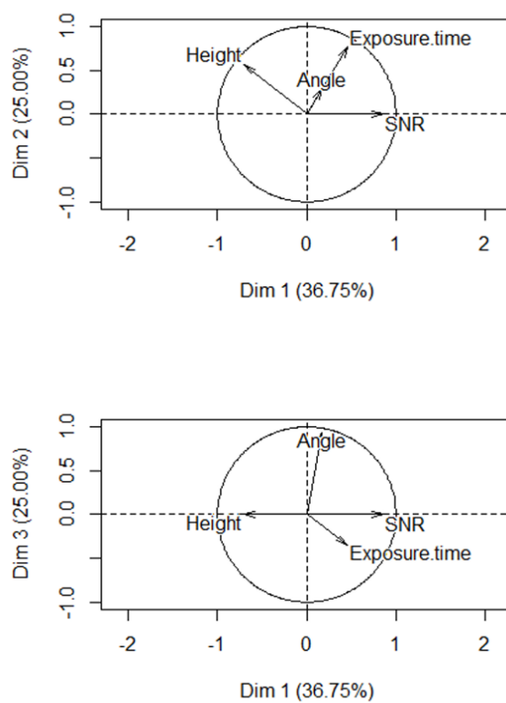
Figure 5. Principal component analysis (PCA) variables factor map plots of a leek canopy, showing the projection on PC1 and PC2 (top) and PC1 and PC3 (bottom). The projection of each variable vector on the axis formed by the signal-to-noise ratio (SNR) vector gives an indication of the relation of this variable to SNR.
