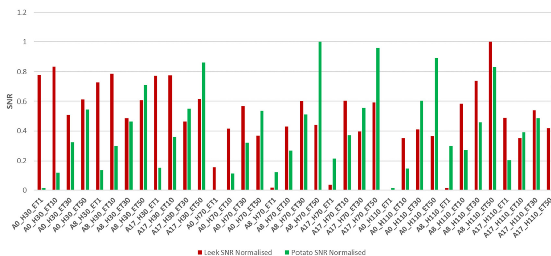
Figure 3. Signal-to-noise ratio (SNR) calculated for the hyperspectral camera for different combinations of setup parameters of height (H), angle (A) and exposure time (ET). Values of SNR were calculated for each wavelength, over all pixels, and then averaged over all wavelengths. Both datasets (leek and potato) have been normalised to be between 0 and 1 using (x-\min)/\text{range} .
