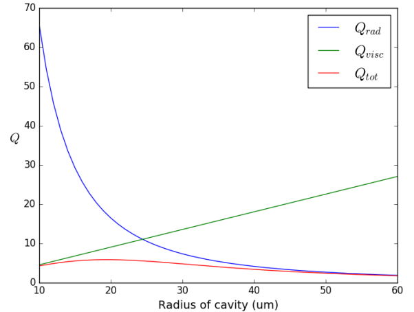
Fig. 2. The total acoustic quality factor is found through Q_{tot}^{-1} = Q_{rad}^{-1} + Q_{visc}^{-1} . This illustrates the competing loss mechanisms and the compromise resulting from it.
