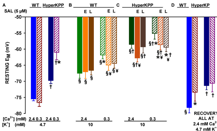
Figure 8. Lowering [Ca 2+ ] e significantly enhanced the K + -induced membrane depolarization in both wild type and HyperKPP soleus. (A) Mean resting E M values were calculated from all tested fibers (mean resting E M of unexcitable and excitable fibers are respectively given in Tables 1 and 2). All [K + ] e and [Ca 2+ ] e conditions are as described in Fig. 7. Data for salbutamol are divided into early measurements (first 10 min, E) and late measurements (15–30 min, L). The reversibility of the K + and Ca 2+ effects was tested by returning to the initial conditions (i.e., 4.7 mM K + and 2.4 mM Ca 2+ ). Vertical bars represent the SE of 71–144 fibers/5–6 muscles for high [K + ] e , 277 fibers/26 muscles for wild type and 273 fibers/18 muscles for HyperKPP at 4.7 mM K + and 2.4 mM Ca 2+ . §, At similar [Ca 2+ ] e , mean resting E M significantly different from that at 4.7 mM K + measured at the beginning of an experiment (i.e., in A). *, At similar [K + ] e , mean resting E M at 0.3 mM Ca 2+ significantly different from that at 2.4 mM Ca 2+ . †, At the same [K + ] e and [Ca 2+ ] e , mean resting E M of HyperKPP fibers significantly different that of wild type fibers. ¥, Significant effect of salbutamol. ANOVA and LSD, P < 0.05.
