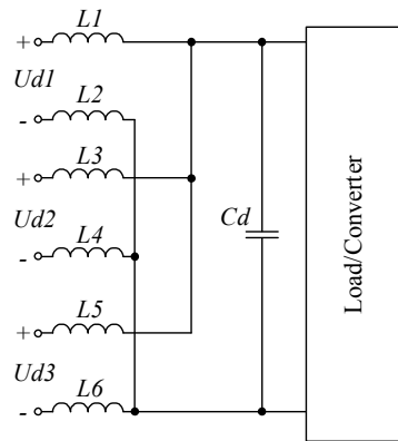
Fig. 12. The single-channel load of 18-pulse converter
