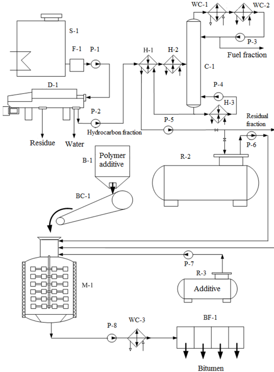
Fig. 2. Technological scheme of modified bitumen production
