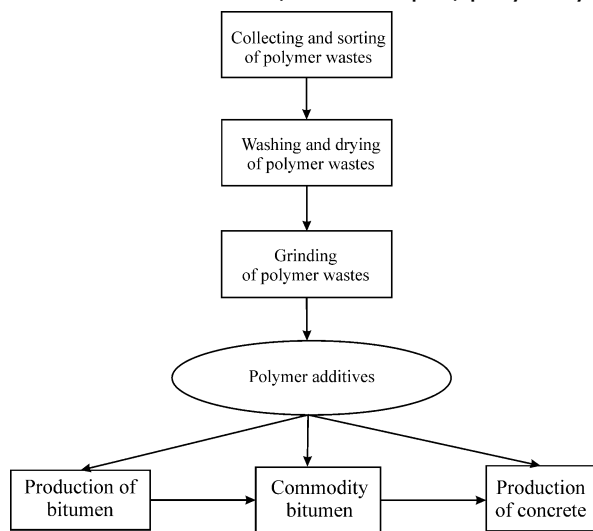
Fig. 1. Structural scheme of modified bitumen production
