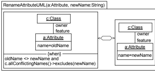
Fig. 3. QVT Formalization of RenameAttribute Refactoring
