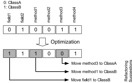
Figure 2: The chromosome structure and usage.
