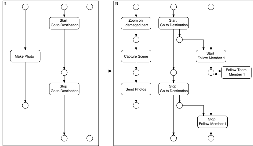
Fig. 7. Parallel rule r = r_{photo} + r_{follow}
