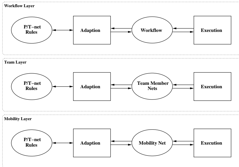
Fig. 11. Layered architecture for supporting cooperative work on MANET
