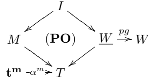
Fig. 12. Consistent layer environment
