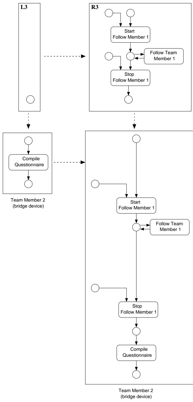
Fig. 6. Rule r_{m2} and its application to t_0^2
