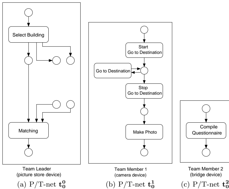
Fig. 2. Team member nets in the team layer
