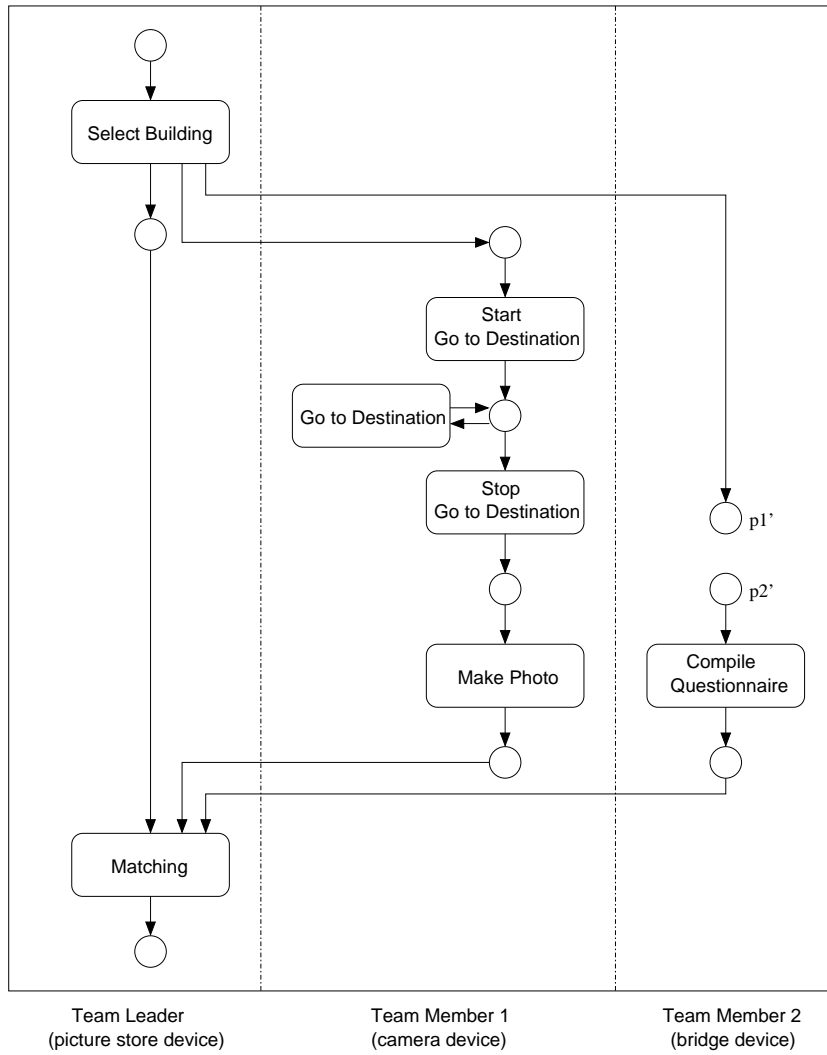
Fig. 3. Teamwork net T_0
