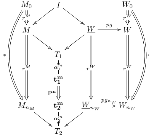
Fig. 21. Restoring the next consistent layer environment
