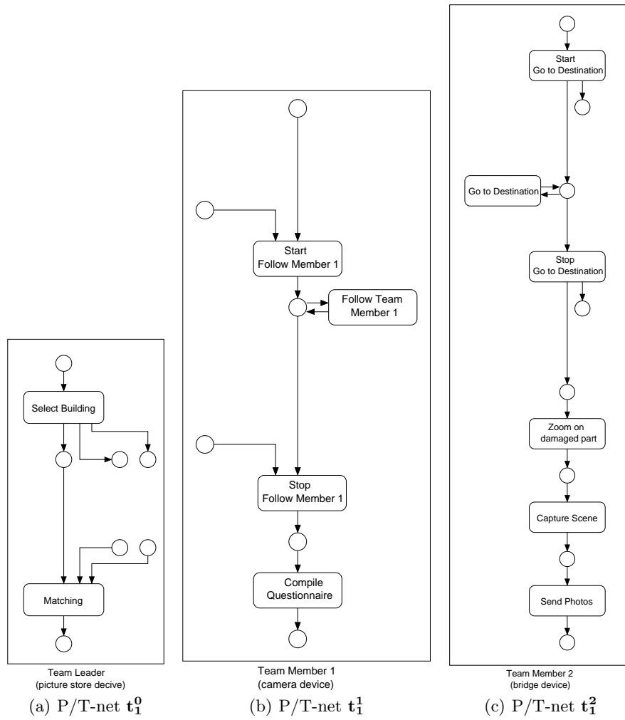
Fig. 8. Team member nets in team layer after rule application
