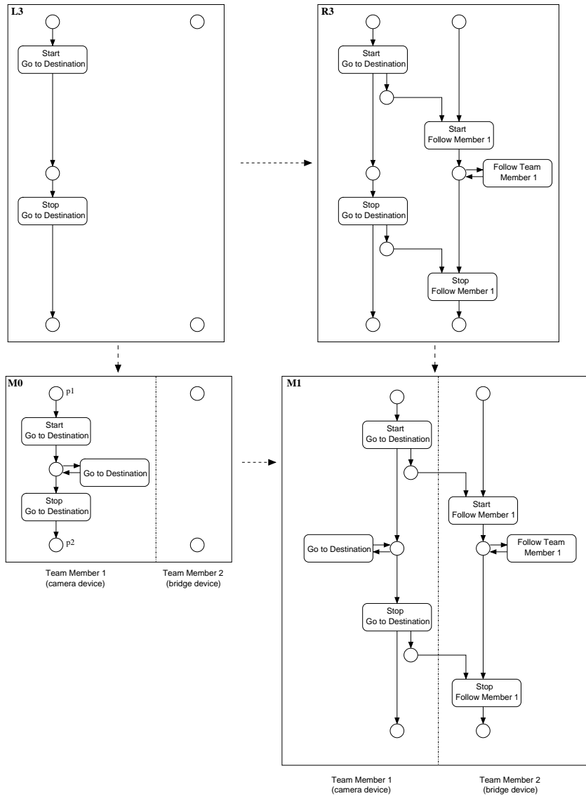
Fig. 5. Rule r_{follow} in the mobility layer and its application
