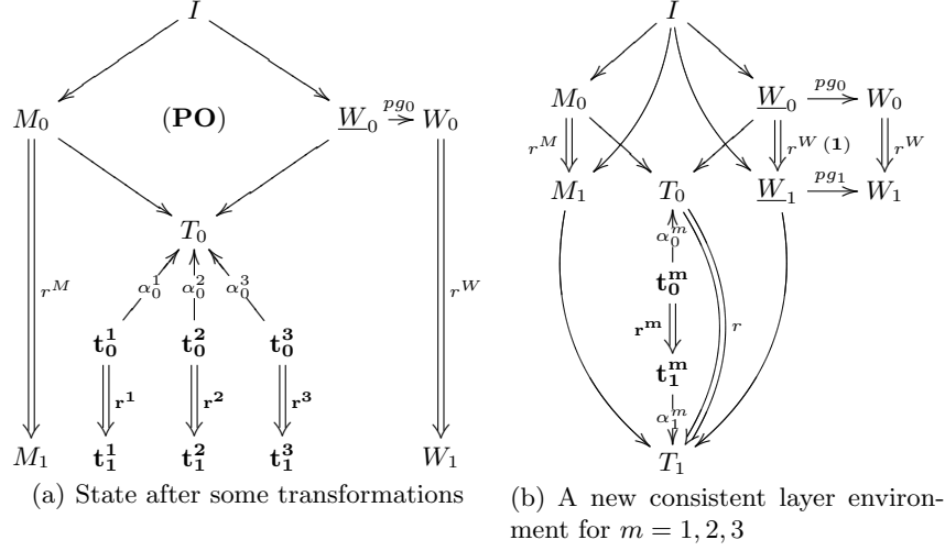
Fig. 13. Layer environment after transformations
