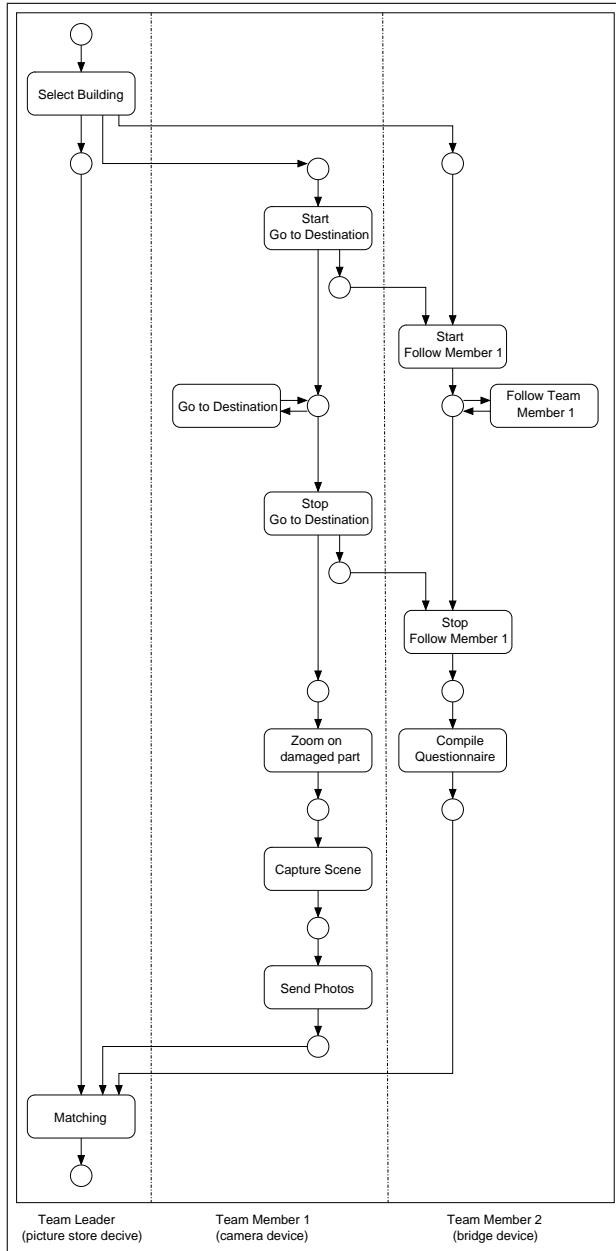
Fig. 9. Teamwork net T_1 after application of rules r_{photo} and r_{follow}
