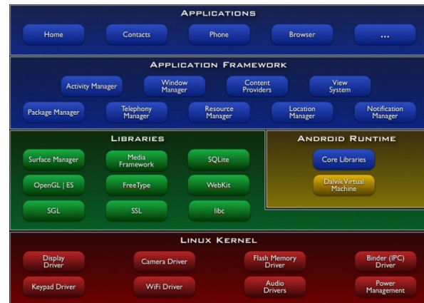
Figure 1: Android system architecture, image courtesy of Google Inc [14].
