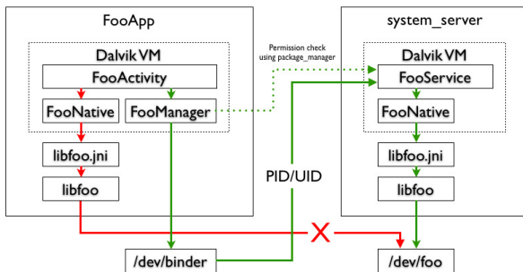
Figure 5: Local permission enforcement on Android is performed by its respective manager.
