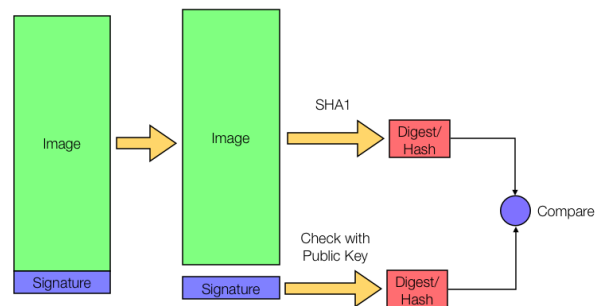
Figure 3: Signature check: The image is hashed while the signature gets decrypted to return the original hash value. Both values then are compared.
