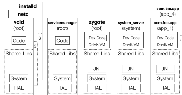
Figure 4: Schematic figure of the processes running in an Android system. Some services run with root privileges which makes them a valuable target for root exploits.
