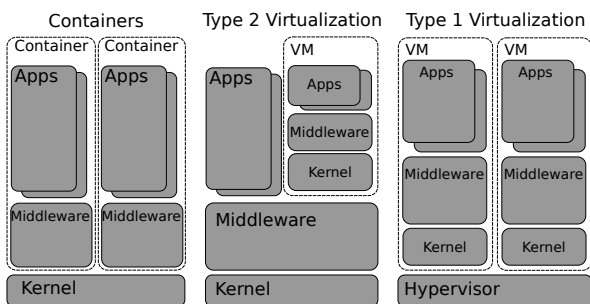
Figure 6: Android virtualization architectures. From left to right: Containers, Type 2 and Type 1 virtualization.
