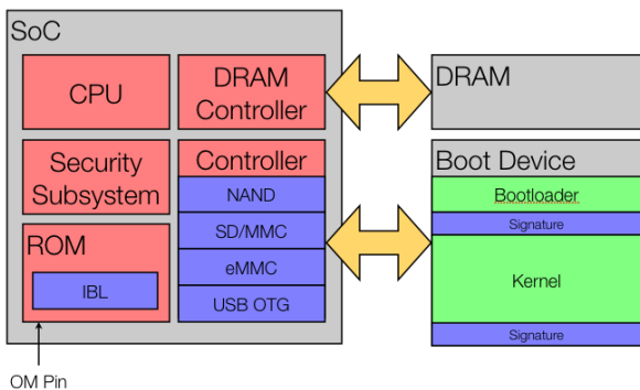
Figure 2: Boot architecture on mobile devices. The OM pin determines the boot medium. The IBL initializes the DRAM and the boot medium controller and loads the bootloader into the RAM. The security subsystem may be used to speed up signature checks.
