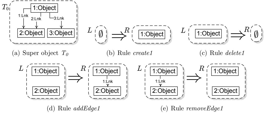
Figure 2: STS \mathcal{S}_0
