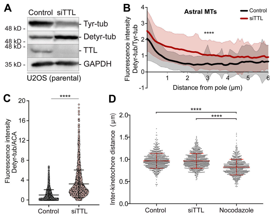
Figure S1. TTL depletion increases \alpha -tubulin detyrosination on astral MTs and in the vicinity of KTs without affecting inter-KT distance. (A) Protein lysates from parental U2OS cells collected 72 h after RNAi transfection in control and after siTTL were immunoblotted for tyrosinated tubulin, detyrosinated tubulin, and TTL. GAPDH was used as loading control. (B) Quantification of the fluorescence intensity ratio between detyrosinated/tyrosinated \alpha -tubulin along astral MTs in control and siTTL metaphase cells ( n = 150 astral MTs/condition; 10 astral MTs/cell, 5 cells/experiment, pool of three independent experiments. ****, P < 0.0001 , unpaired two-tailed t test). (C) Quantification of the fluorescence intensity of detyrosinated \alpha -tubulin relative to ACA at the KTs in control siTTL U2OS cells ( n [control] = 2,224 KTs, 19 metaphase cells, pool of two independent experiments; n [siTTL] = 2,507 KTs, 19 metaphase cells, pool of two independent experiments. ****, P < 0.0001 , unpaired two-tailed t test). The mean fluorescence intensity of tubulin detyrosination at KTs normalized by the mean of control cells is represented. Error bars represent SD. (D) Quantification of the inter-KT distance in control, siTTL, and nocodazole ( 1 \mu\text{M} )-treated U2OS parental cells ( n [control] = 762 KT pairs, n [siTTL] = 795 KT pairs, and n [nocodazole] = 695 KT pairs, from 6–11 cells/condition, pool of three independent experiments. ****, P < 0.0001 , unpaired two-tailed t test).
