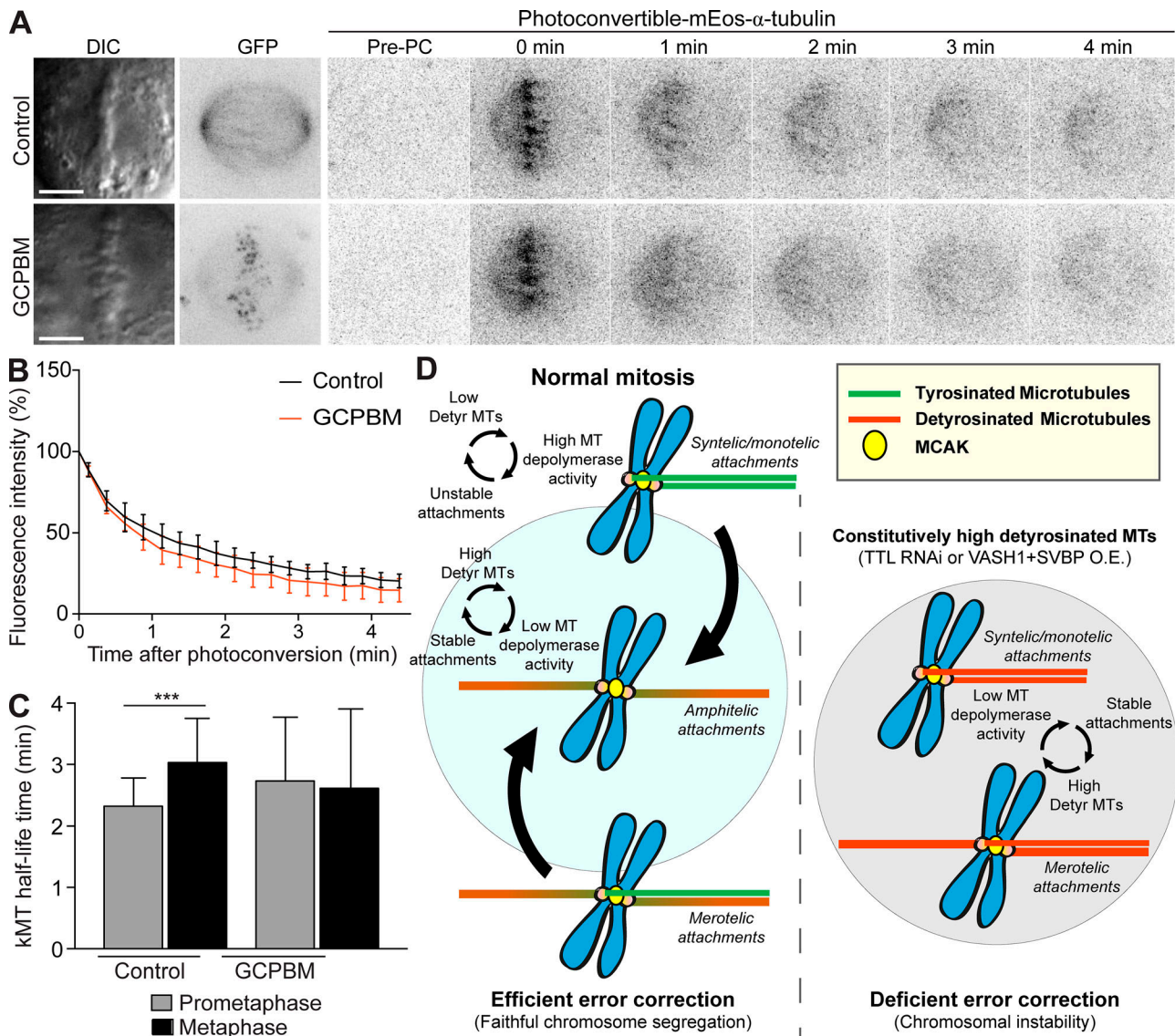
Figure 7. Centromeric MCAK does not significantly alter global kMT dynamics. (A) Representative images of DIC and time-lapse fluorescent images of metaphase spindles of U2OS cells stably expressing mEos- \alpha -tubulin. Photoconversion was performed after overexpression of GFP (control) and GCPBM. Images before photoconversion (Pre-PC) and at the indicated times points (min) after photoconversion are displayed. Scale bars, 5 \mu m. (B) Normalized fluorescence intensity after photoconversion of mEos- \alpha -tubulin in U2OS cells in metaphase (GFP-control: n = 9 cells from five independent experiments and GCPBM: n = 6 cells from three independent experiments). Data points represent mean \pm SD. (C) Calculated kMT t_{1/2} in control and GCPBM-overexpressing cells in prometaphase (GFP-control: n = 21 cells, and GCPBM: n = 25 cells, pool of five independent experiments, P = 0.0847 , unpaired two-tailed t test) and metaphase (GFP-control: n = 9 cells from five independent experiments and GCPBM: n = 6 cells from three independent experiments, P = 0.4351 , unpaired two-tailed t test) using the fluorescence decay after photoconversion. Only kMT t_{1/2} between prometaphase and metaphase in control cells varied significantly. ***, P < 0.001 . Bars indicate mean values/cell, and error bars represent SD. (D) Proposed model for the discrimination of mitotic errors by MT detyrosination (see Discussion for description). O.E., overexpression.
