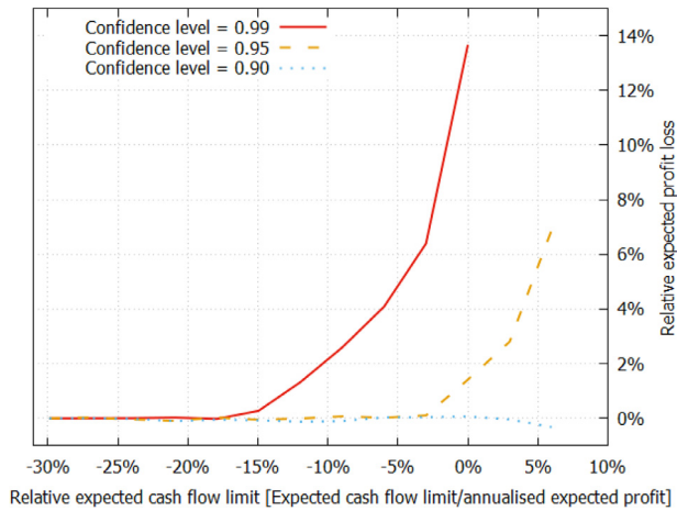
Fig. 6. The efficient frontiers for the CVaR model solved for the large instance with correlated random variables and normal space charter price. Let E^* be the annualized expected profit without cash flow control, and E^{\bar{F}_\alpha} the annualized expected profit using cash flow threshold \bar{F}_\alpha . The vertical axis represents the ratio 100 * (E^* - E^{\bar{F}_\alpha})/E^* . The relative expected cash flow limit is calculated as the minimum expected cash flow allowed, \bar{F}_\alpha , divided by the annualized expected profit.
