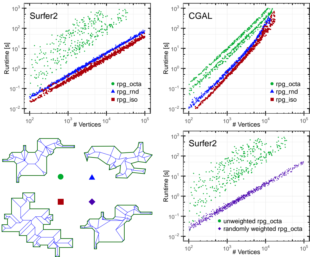
■ Figure 9 Top: The effect of different input classes on the runtime of SURFER2 and on CGAL. Bottom-left: Samples for different input classes (left to right, top to bottom): Octagonal input (on integer grid), random polygon, orthogonal polygon not on integer grid, and weighted octagonal input. Bottom-right: SURFER2 runtimes for unweighted and randomly weighted octagonal input.
