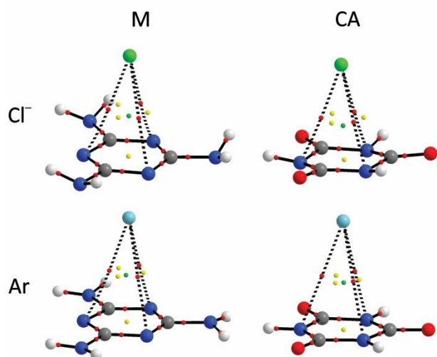
Fig. 5 Molecular graphs of M\cdots Cl^-/Ar and CA\cdots Cl^-/Ar complexes. Small red dots are BCP, yellow dots are ring critical points and green dots are cage critical points.
