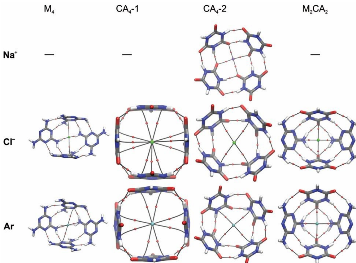
Fig. 6 Molecular graphs of multimolecular inclusion compounds.
