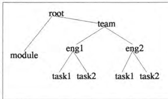
Figure 3.11: Composite-Object Hierarchy
