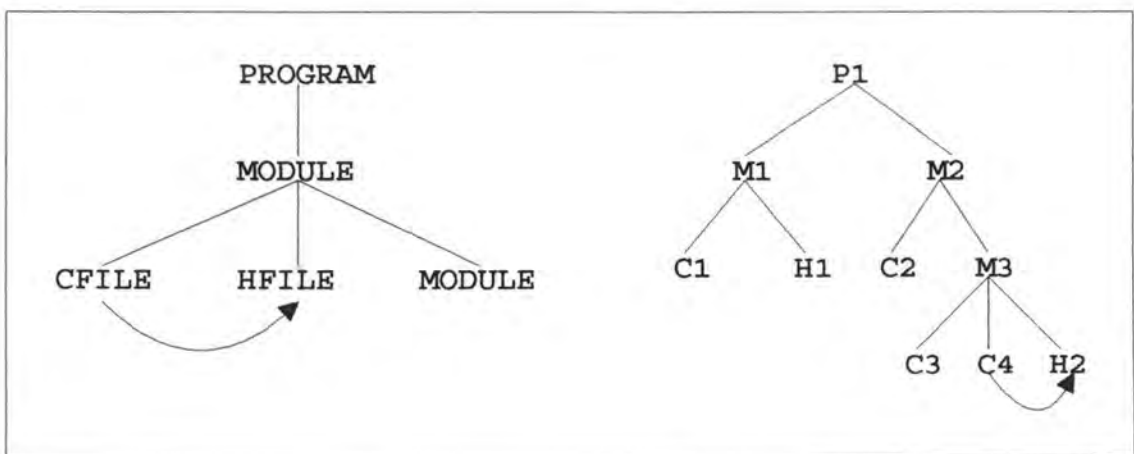
Figure 2.4: Composite Hierarchy
