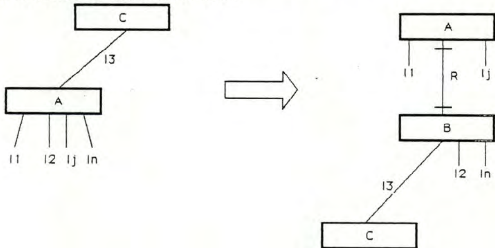
Figure 7.43: Eclatement/fusion de types d'articles.
