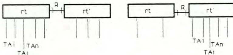
Figure 3.2: Transfert de types d'associations entre RECORD-TYPES.
