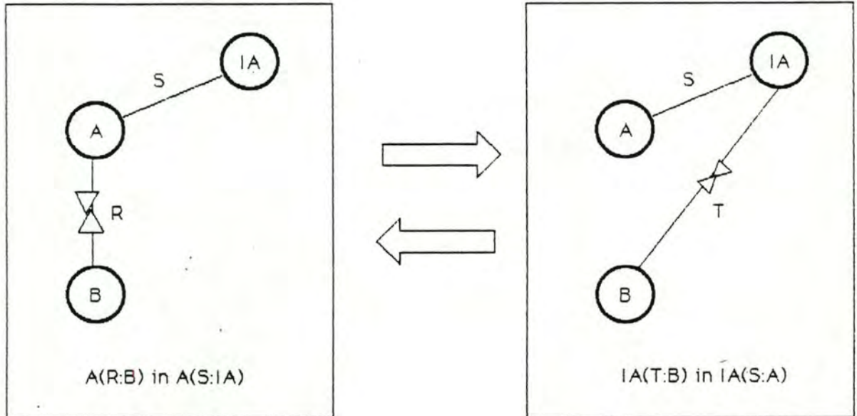
Figure 7.4: Rotation de types d'associations.
