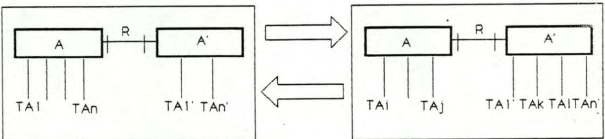
Figure 7.6: Transfert de types d'associations.
