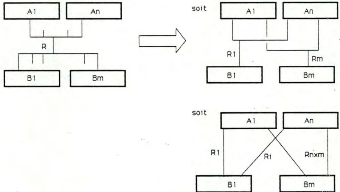
Figure 7.41: Eclatement/fusion de types de chemins.
