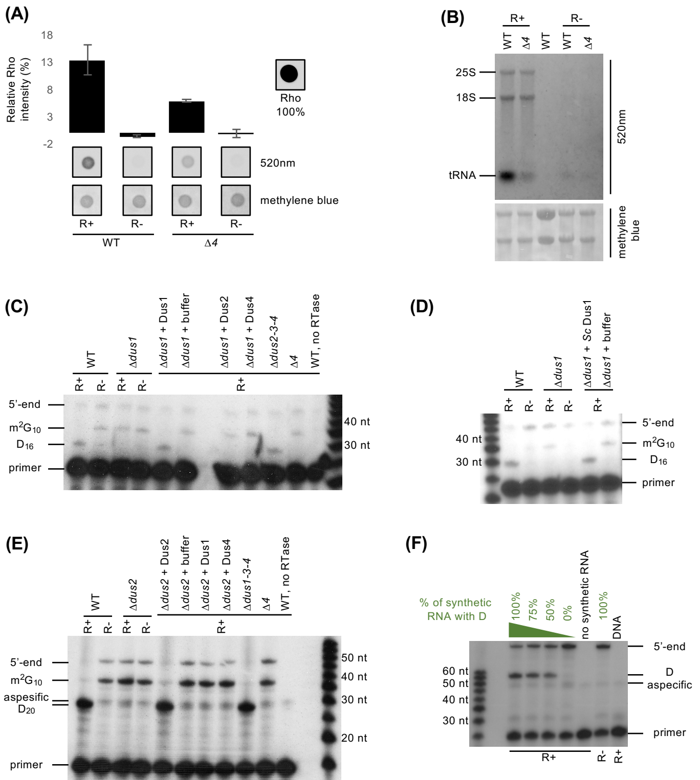
Figure 10 – Single-nucleotide detection of dihydrouridine (D) by rhodamine labeling. (A) Comparative Rho (rhodamine) detection at 520nm on WT (wild type) and \Delta 4 ( \Delta dus1-2-3-4 ) total RNAs in R+ and mock-treated (R-) samples. The intensity of a Rho drop is scaled at 100%, a drop of water is considered as the background, methylene blue staining serves as loading control, n = 3 , error bars represent SEM. (B) Fluorescent Northern blotting of WT and \Delta 4 total RNAs in R+ and mock-treated samples. Untreated total RNA from WT strain is shown in lane 3. Representative result from a biological triplicate, methylene blue staining serves as loading control. (C-D-E) Primer extension assays performed on total RNAs from WT, single dus ( \Delta dus1 , \Delta dus2 ), triple dus ( \Delta dus1-3-4 , \Delta dus2-3-4 ) or quadruple dus ( \Delta 4 ) mutant strains, R+ or R- treated. Before the chemical reaction, in vitro dihydrouridylations are performed with S. pombe GST-purified proteins (+ Dus1, 2 or 4), S. cerevisiae GST-purified Dus1 (+ Sc Dus1) or no protein (+ buffer) on S. pombe total RNA from different genetic backgrounds. The ladder consists of ^{32}P -labeled DNA oligonucleotides ranging from 15 to 60 nt. (C-D) primer specific for tRNA^{Met} , (E) primer specific for tRNA^{AspGUC} . (F) Primer extension assay performed on an in vitro transcribed RNA mixed with S. pombe total RNA. In green, decreasing amount of dihydrouridylated and increasing amount of uridylated synthetic RNAs are added before R+ or R- chemical reactions. DNA is the PCR product used for in vitro transcription.
