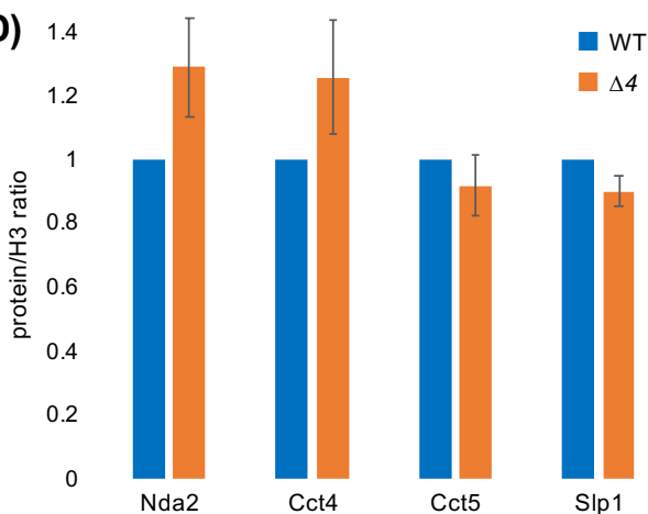
Figure 19 – Transcriptomic and protein analyses of the \Delta 4 mutant. (A) Significantly and differentially expressed genes revealed by RNA-seq on WT and \Delta 4 total RNA samples. On the left , list of downregulated genes in the quadruple dus mutant. On the right , list of upregulated genes in the quadruple dus mutant. logFC stands for \log_2 (fold change). (B) Volcano plot highlighting all tRNA genes (red dots) and all other fission yeast transcripts (black dots) mapped in the RNA-seq experiment. (C) qRT-PCR analyses ( \Delta\Delta C_T method) on D-seq candidates whose protein products are targeted by the CCT folding complex (green V) or not (red cross), are cytoskeletal proteins (green V) or not (red cross). 25S rRNA is a noncoding transcript control, nab3 is a coding transcript control, WT expression values (blue) are scaled to 1 (au, arbitrary units), \Delta 4 expression mean values are in orange, n = 3 , error bars represent SEM, normalization is done on adh1 expression. (D) Relative protein expression of one D-seq candidate ( Nda2 ), two tagged CCT subunits ( Cct4 and 5 ) and one target of the CCT complex ( Slp1 ). Histone H3 is used as a loading control. On the left , ratio (protein of interest/H3) is scaled at 1 for WT (blue) and variations are shown for the \Delta 4 mutant (orange), n = 3 , error bars represent SEM. On the right , representative result of a Western blotting triplicate against Nda2 (upper left, anti- Nda2 Ab – antibody), Cct4/5-TAP (upper middle, anti-TAP Ab), Slp1-HA (upper right, anti-HA Ab) and H3 (lower, anti-H3 Ab) in different genetic backgrounds. For C and D, Student's t -tests were performed (on the Cq values or on the ratio (protein of interest/H3), respectively) and differences between WT and mutant were all non-significant ( p > 0.05 ).
