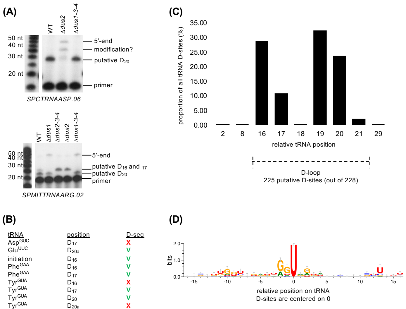
Figure 14 – D-seq detects D on yeast tRNAs. (A) Primer extension assays performed on R+ total RNAs from WT, single dus ( \Delta dus1 , \Delta dus2 ) and triple dus ( \Delta dus1-3-4 , \Delta dus2-3-4 ) mutant strains. D-seq analysis suggested U 20 modification on SPCTRNAASP.06 and U 16 , 17 and 20 modifications on SPMITTRNAARG.02 , that are all confirmed here. Above ; primer specific for tRNA Asp GUC , below ; primer specific for mitochondrial tRNA Arg UUC . (B) List of known D positions and their cognate tRNAs in S. pombe . Last column indicates the detection of the corresponding position (green V) or not (red cross) in the D-seq analysis. (C) Distribution of the 228 tRNA D-sites according to their relative position on tRNA. Unlike in Fig. S9, the D-sites were not manually curated to be assigned to a canonical D-site (D 16 , 17, 20, 20a or 47). (D) Consensus sequence surrounding the 228 tRNA D-sites.
