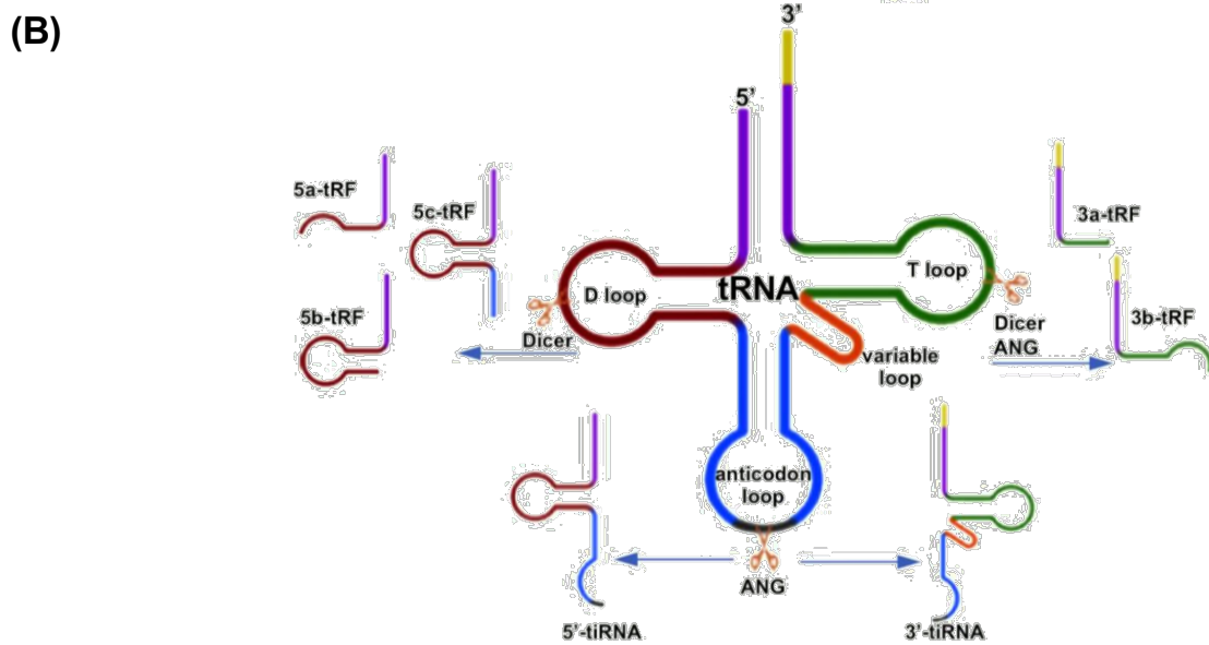
Figure 2 – Functional noncoding RNAs. (A) MALAT1 is a processed long noncoding RNA; a 61nt-long RNA (mascRNA) is exported to the nucleus and a 7kb-long RNA (mature MALAT1) adopts a stable 3'-triple helix to be localized to the nuclear speckles (Quinn and Chang, 2016). (B) tRNA-derived small tRNAs are classified into two classes; tRf (tRNA-derived fragment) and tiRNA (tRNA-derived stress induced RNA). The cleavage is performed on different tRNA positions by ribonucleases such as Dicer or angiogenin (ANG) (Li et al., 2018).
