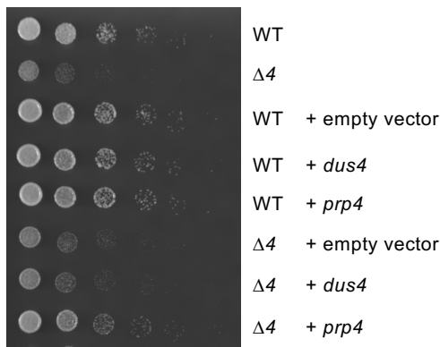
Figure 24 – Phenotyping the yeast \Delta 4 mutant. (A) Sensitivity of the quadruple S. pombe \Delta 4 mutant was assessed by spot assay and compared to the WT growth in all listed conditions. Asterisks indicate that the mutant was more sensitive than the WT strain but most likely in dus -independent manner, as exemplified in (B) . MT (microtubule). (B) Growth phenotype of the \Delta 4 mutant compared to the WT strain. Exponential growing cells were spotted on rich medium supplemented with 12.5µg/mL of thiabendazole (TBZ) and incubated at 32°C (5-fold dilutions). All strains carried an auxotrophic marker for the positive selection of the vector during (pre-)culturing growth in a defined medium. The vector used in this study resulted in the overexpression of the cloned gene ( dus4 or prp4 ).
