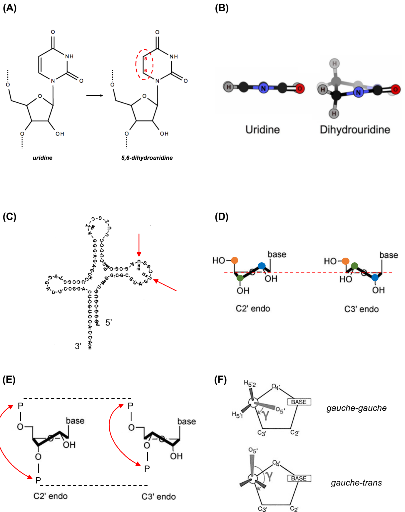
Figure 4 – Biochemistry of dihydrouridine. (A) Reduction of uridine into dihydrouridine. (B) Dihydrouracil is a nonplanar nucleobase (carbon in black, nitrogen in blue, oxygen in red and hydrogen in gray) (Whelan et al., 2015). (C) First published structure of a ribonucleic acid (yeast tRNA Ala ) where D (red arrows) are shown in a loop at the 5'-end (Holley et al., 1965). (D) Schematic representation of ribose pucker. C5' (orange dot) is considered as being above the C4'-O'-C1' plane (red dashed line). On the left , C2'-endo has the C2' (blue dot) above the plane. On the right , C3'-endo has the C3' (green dot) above the plane (Moreau et al., 2011). (E) C2'-endo pucker produces a longer 5'-phosphate/3'-phosphate distance and therefore spans the polynucleotide (Moreau et al., 2011). (F) Schematic representation of ribose gauche-gauche and gauche-trans conformations. C5' (white dot) adopts different torsion angles ( \gamma ) that modulate the positioning of C5'-bound atoms (H 5'1 , H 5'2 and O 5' ) (Saenger, 1984).
