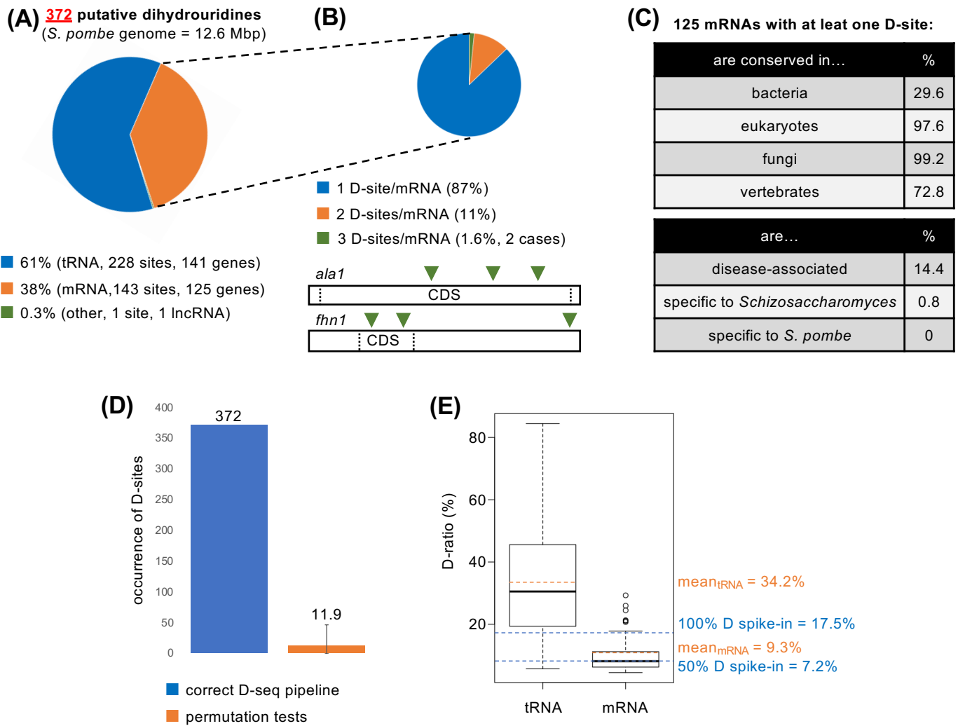
Figure 17 – Yeast protein-coding genes products are dihydrouridylated. (A) Repartition of 372 detected D-sites in fission yeast on three distinct RNA species; transfer, messenger and long noncoding RNAs. (B) Putatively dihydrouridylated mRNAs had up to three distinct D-sites on their sequence. ala1 (coding for an alanine-tRNA ligase) and fhn1 (coding for an eisosome assembly factor) are the two mRNAs dihydrouridylated at three different positions (green triangles). The CDS (coding DNA sequences) are delimited with black dashed lines. (C) Diverse features of the 125 protein coding-genes whose RNA products were modified. (D) Correct assignment of test and control conditions was essential in the D-seq analysis pipeline. Sixteen permutation tests were performed in which the properly committed information 1_WT R+; 2_WT R-; 3_Δ4 R+; 4_Δ4 R- (blue bar, 372 D-sites) was randomly mixed into, for example, 1_WT R-; 2_Δ4 R-; 3_Δ4 R+; 4_WT R+ (orange bar, average of 11.9 D-sites, error bars represent max and min numbers of detected D-sites). (E) Box plot representation of WT R+ D-ratios distribution for tRNAs (228 values) and mRNAs (143 values) and corresponding means highlighted by orange dashed lines (note: this is different from the mean of the D-ratio as presented in Fig. 12, which summarizes the information from test and control conditions). Blue dashed lines indicate the D-ratios of R+ D 100% spike-in (Fig. 13A) and D 50% spike-in (Fig. 13F).
