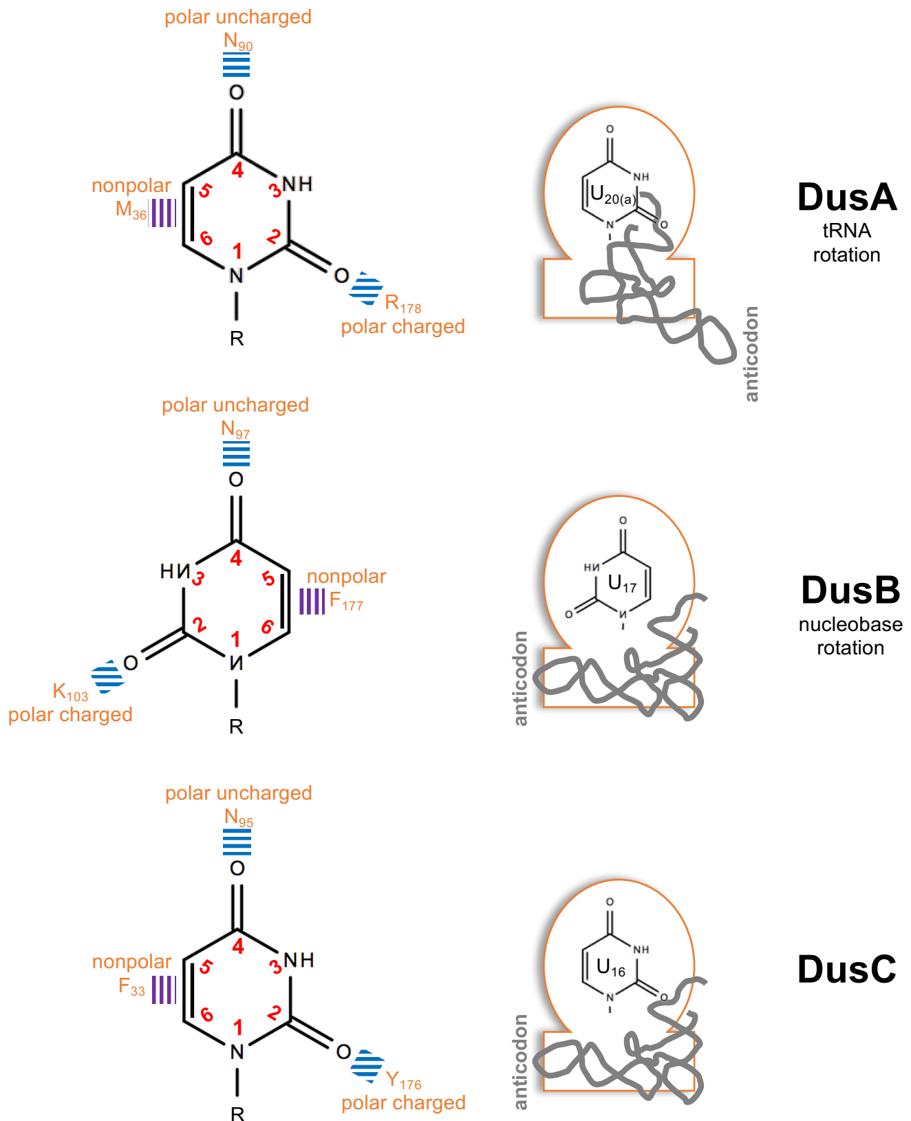
Figure 8 – Molecular strategies of bacterial Dus enzymes for substrate specificities. On the left, interaction of the U nucleobase (in the context of the RNA chain (R)) with Dus amino acids (orange: F for Phe, N for Asn, K for Lys and Y for Tyr) through ionic (blue lines) or hydrophobic (purple lines) interactions. In the DusB catalytic pocket, the rotation of the U nucleobase ( 180^\circ ) is observed in comparison to the DusA and C counterparts. On the right, schematic representations of the Dus enzymes (orange line) with the N-terminal nucleobase-containing catalytic domain (round) and the C-terminal RNA binding domain (rectangle). The tRNA (gray line) docking is similar in DusB and C but differs by a rotation ( 160^\circ ) in DusA. These strategies (tRNA or nucleobase rotations) allow the unvariable targeting of a specific uridine.
