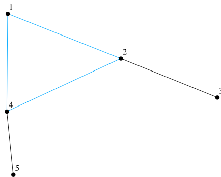
Figure 3.4: Cycle
