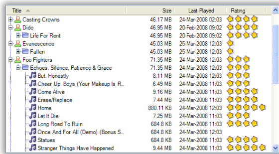
Figure 4.1: Treeview [Gra15]
