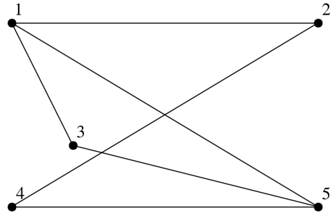
Figure 3.11: Dessin non-planaire
