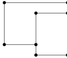
Figure 3.13: Dessin orthogonal
