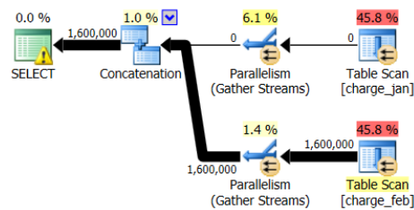
Figure 4.2: Graphe [Sac15]
