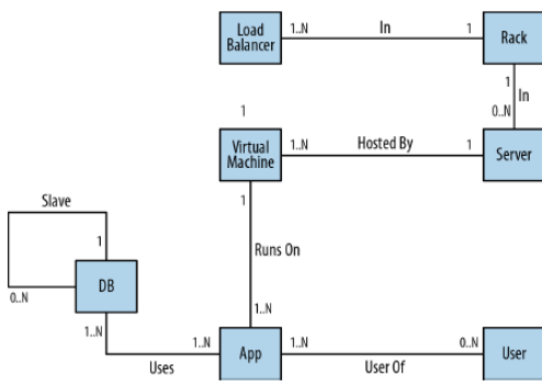
Figure 3.36: Cardinalités [IR15]
