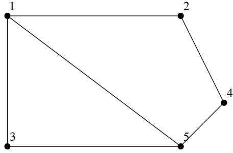
Figure 3.10: Dessin planaire
