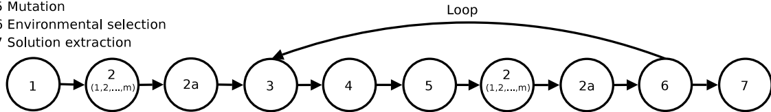
Figure 2.13: Generalized MOEA sequential task decomposition (adapted from [13]).
