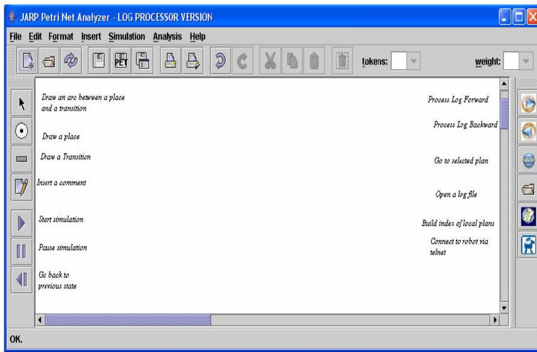
Fig. 7.21: Jarp windows
