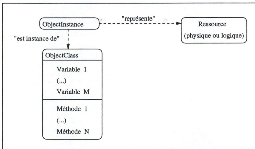
FIG. 3.4 – ObjectInstance .
