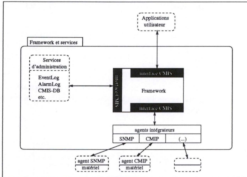
FIG. 1.10 – Architecture d'OPENMASTER.
