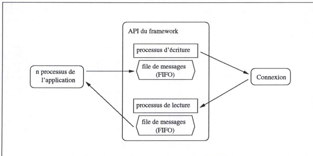
FIG. 5.5 – Seconde solution asynchrone.
