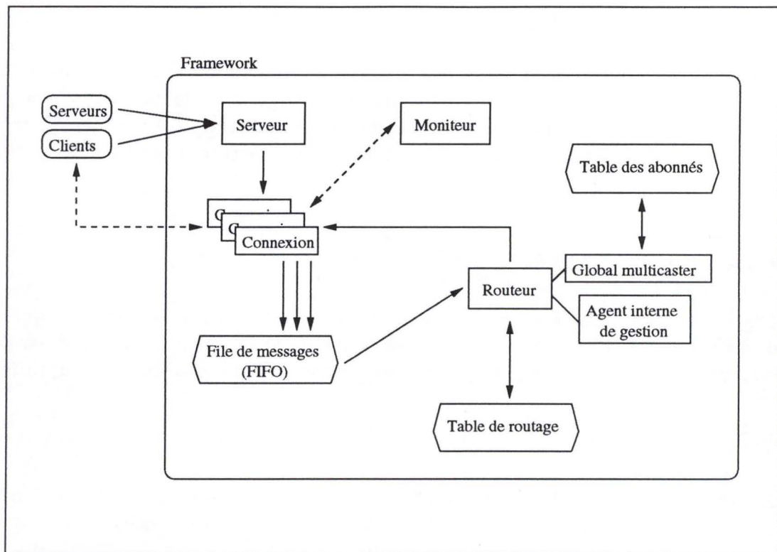
FIG. 4.5 – Architecture du framework.
