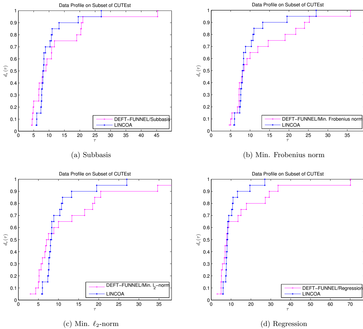
Figure 5.6: Data profiles of the methods DEFT-FUNNEL (with different approaches to build the models) and LINCOA on a set of 20 linearly constrained problems from CUTEst.
