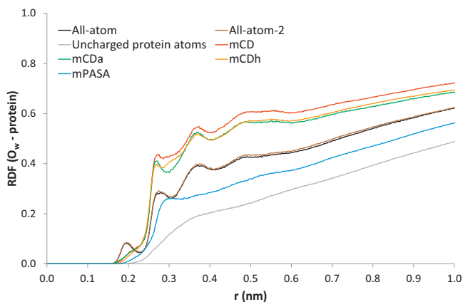
Fig. 8. RDF of water oxygen-protein atom pairs of the solvated system Vps27 UIM1-Ubiquitin calculated from the last 10 ns of the Amber99SB-based MD trajectories at 300 K, as obtained using the All-atom, All-atom-2, mCD, mCDa, mCDh, mPASA, and neutral protein atom models. (For an interpretation of the references to colour in the artwork, the reader is referred to the web version of the article).
