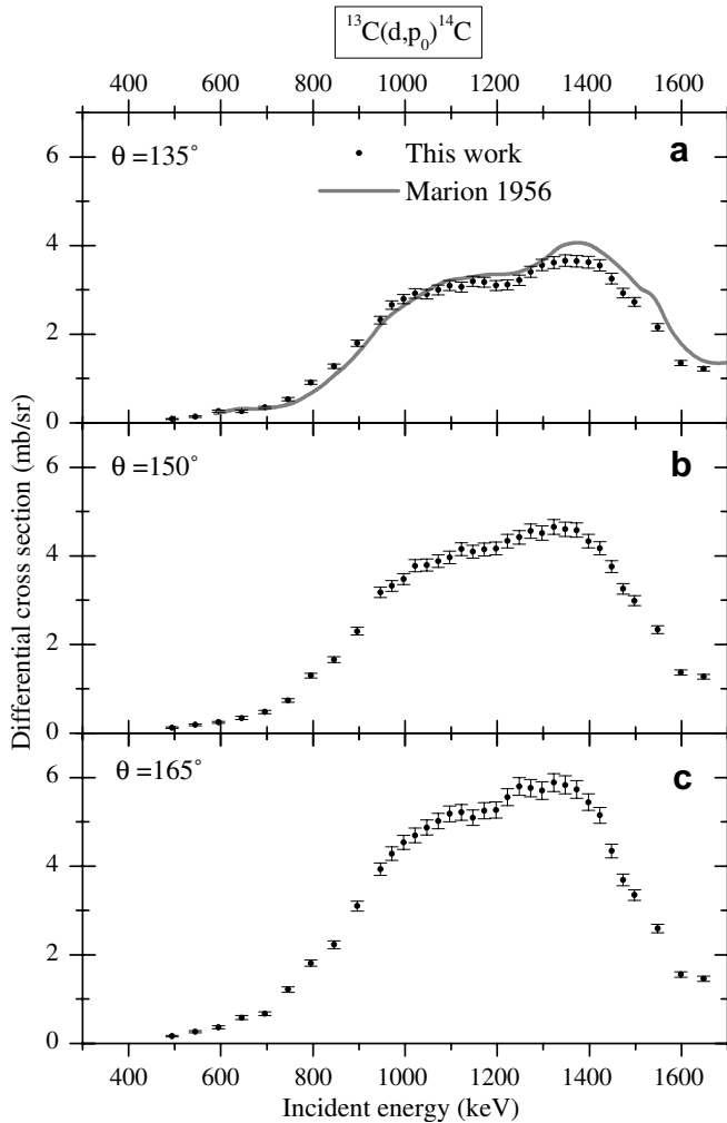
Fig. 2. Differential cross section curves for ^{13}\text{C}(d, p_0)^{14}\text{C} nuclear reaction measured at 135° (a), 150° (b) and 165° (c) in the laboratory system. Symbols (filled circles) represent the measurements performed in this work while the solid line represents measurements made by Marion and Weber [3].
