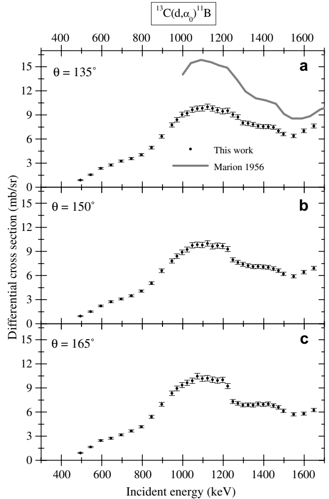
Fig. 3. Differential cross section curves for ^{13}\text{C}(d, \alpha_0)^{11}\text{B} nuclear reaction measured at 135° (a), 150° (b) and 165° (c) in the laboratory system. Symbols (filled circles) represent the measurements performed in this work while the solid line represents measurements made by Marion and Weber [4].
