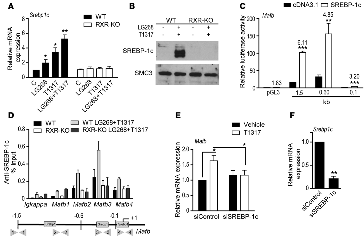
Figure 8. RXR/LXR induces Mafb transcription through SREBP-1c. (A) Srebp1c mRNA expression in WT and RXR-KO osteoclast progenitors treated with vehicle (C) or ligands for RXR (LG268) and LXR (T1317). * P < 0.01 ; ** P < 0.001 , compared with WT vehicle-treated cells (C). (B) SREBP-1c protein expression in nuclear extracts from osteoclast progenitors treated with vehicle or ligands for RXR (LG268) and LXR (T1317); SMC3 was used as loading control. (C) Luciferase reporter assay in RAW264.7 cells transfected with SREBP-1c or empty cDNA3.1 vector together with the indicated Mafb promoter or pGL3 control reporters; data are presented relative to values obtained with the vehicle-treated pGL3 reporter in the absence of SREBP-1c (cDNA3.1). Indicated fold inductions represent (SREBP-1c)/(cDNA3.1). ** P < 0.01 ; *** P < 0.001 , compared with reporter activity in the absence of SREBP-1c. (D) ChIP analysis of SREBP-1c binding to -1.5 kb ( Mafb1 ), -1.0 kb ( Mafb2 ), -0.4 kb ( Mafb3 ), and transcription starting ( Mafb4 ) regions of the Mafb promoter or to a negative control ( Igkappa ) in osteoclast progenitors. Lower panel, localization of SREBP-1c-binding sites in the Mafb promoter. Arrows indicate the position of primers used for ChIP; the experiment shown is representative of 3 done in triplicate. mRNA expression of Mafb (E) and Srebp1c (F) in osteoclast progenitors transfected with control siRNA (siControl) or Srebp1c siRNA (siSREBP-1c). Data are presented as mean \pm SEM ( n = 3 per group). * P < 0.01 ; ** P < 0.001 , by paired (A) or unpaired (C, E, and F) 2-tailed Student's t tests.
