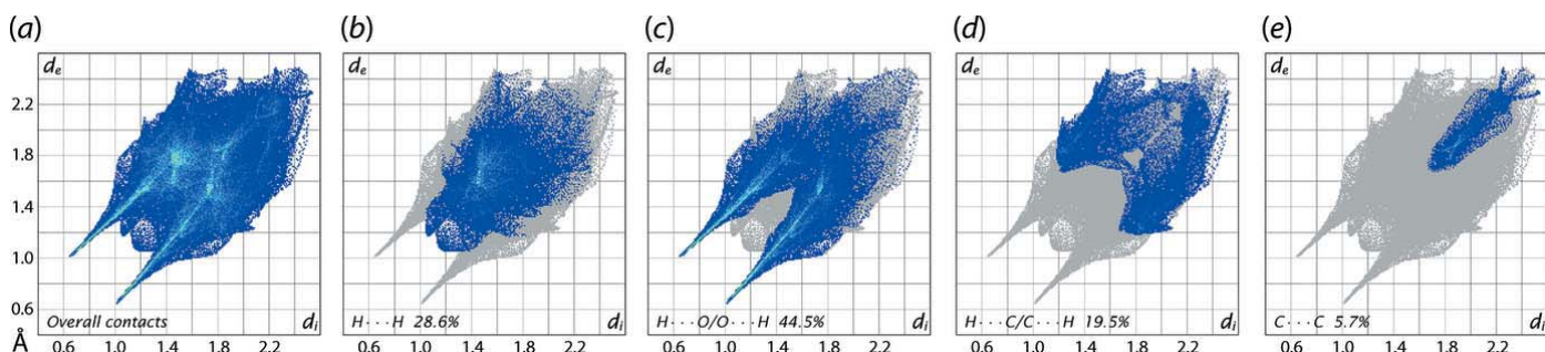
Figure 6 (a) The overall two-dimensional fingerprint plots for (I), and those delineated into (b) H...H, (c) O...H/H...O, (d) C...H/H...C and (e) C...C contacts.
