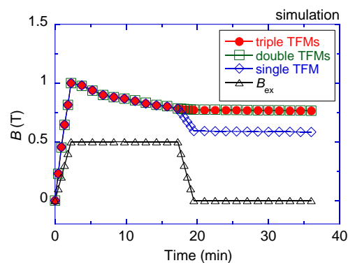
Figure 7. The numerical simulation results of magnetic field, B_c , during the magnetizing process for B_{app} = 0.5 T at the centre of the HTFML using triple, double and single EuBaCuO TFM.
