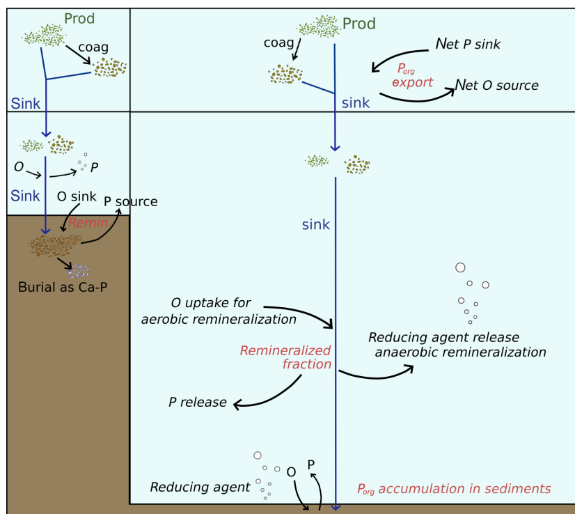
Figure 2. Representation of the physical and biogeochemical fluxes affecting the P_{\text{org}} cycling in the model. Even though some processes (such as burial as Ca–P) are here represented in detail only in one box, the set of biogeochemical processes regulating the P_{\text{org}} dynamics in shelf sea and open ocean (both water column and sediments) is the same, as described in Sect. 2.2.
