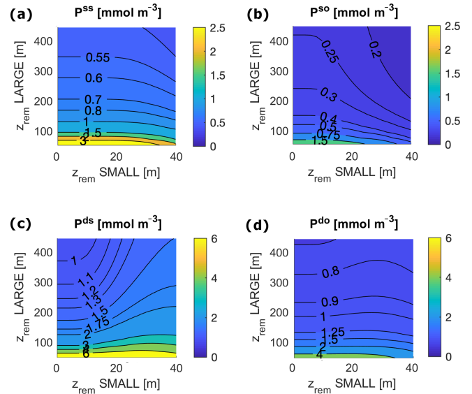
Figure 5. Local P concentration in each ocean box for varying z_{\text{rem}}^{\text{S}} and z_{\text{rem}}^{\text{L}} for the following: (a) surface shelf sea, ss; (b) surface open ocean, so; (c) deep shelf sea, ds; and (d) deep open ocean, do. Surface ocean boxes, as well as deep ocean boxes, are plotted on the same scale.
