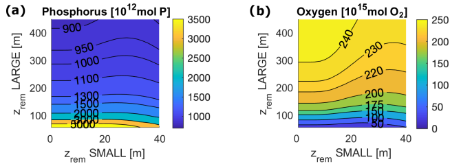
Figure 4. Total ocean budgets of (a) P and (b) O at equilibrium for varying z_{\text{rem}}^{\text{S}} and z_{\text{rem}}^{\text{L}} .
