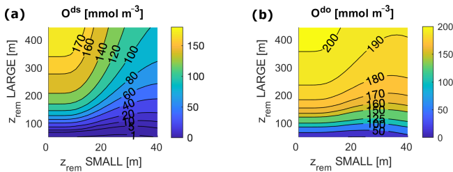
Figure 6. O concentrations at equilibrium for varying z_{\text{rem}}^{\text{S}} and z_{\text{rem}}^{\text{L}} for the following: (a) deep shelf sea, ds; (b) deep open ocean, do. Surface ocean boxes (not shown) have nearly constant values of O for any set of z_{\text{rem}} due to the air–sea gas exchange, which strongly couples them to the atmosphere.
