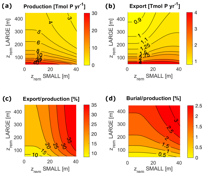
Figure 7. Biological pump fluxes in P units for the entire ocean for varying z_{\text{rem}}^{\text{S}} and z_{\text{rem}}^{\text{L}} in the following cases: (a) P_{\text{org}} surface production; (b) P_{\text{org}} export through the euphotic layer depth; (c) export / production, i.e. export to production ratio; and (d) burial to production ratio.
