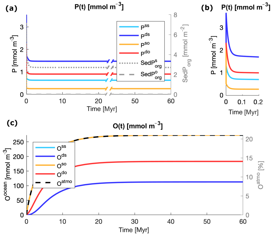
Figure 3. Evolution of the state variables from the initial conditions listed in Table 2 and remineralization lengths roughly in the middle of the interval of explored values, z_{\text{rem}}^{\text{S}} = 20 m and z_{\text{rem}}^{\text{L}} = 250 m. (a) Evolution of inorganic phosphorus P in the water column (left axis) and of organic phosphorus in the sediments \text{SedP}_{\text{org}} (right axis). (b) A zoomed-in view of the dynamics of P in the first 200 000 years. (c) Evolution of oxygen in the water column (left axis) and atmosphere (right axis). In (c) the two lines O^{\text{ss}} and O^{\text{so}} are overlapping; the two variables evolve closely due to the coupling of the surface ocean with the atmosphere via air–sea gas exchange.
