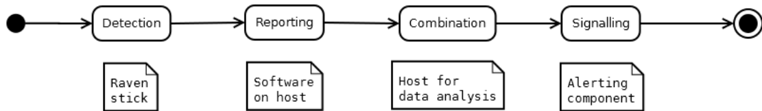
Figure 5.3: Honeypot sketch
