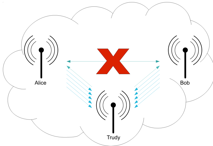
Figure 2.5: Sinkhole attack
