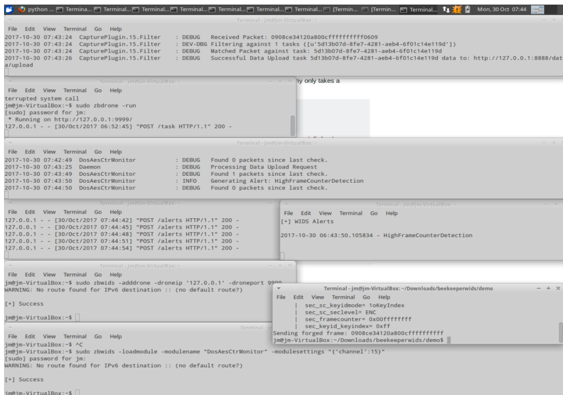
Figure 6.2: MAC layer attack detection example
