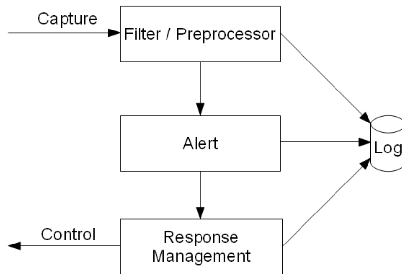
Figure 3.2: Honeypot working scheme
