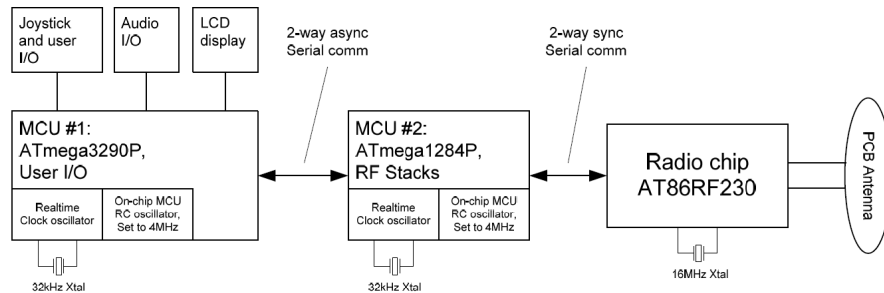
Figure 5.8: Diagram of AVR Raven module
