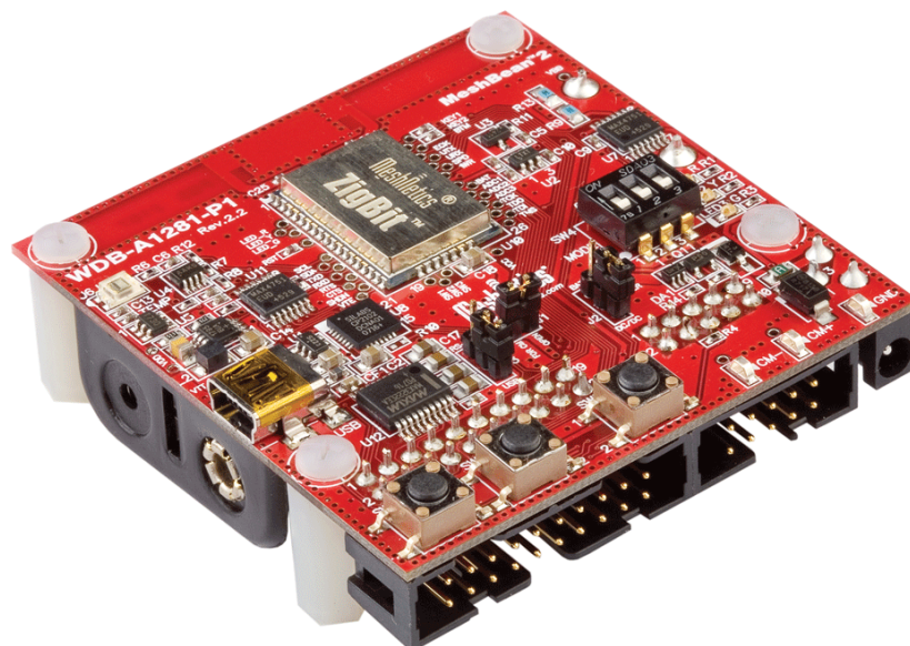
Figure 5.6: Meshnetics MeshBean2 board with ZigBit module
