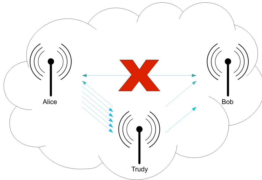
Figure 2.4: Selective forwarding
