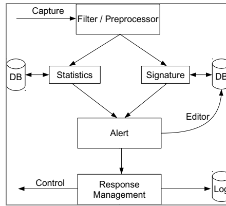
Figure 4: Intrusion detection system (IDS) working scheme
