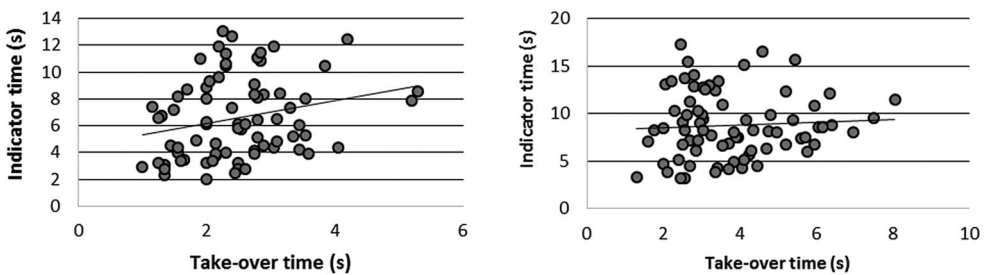
Figure 14. Correlation between the indicator time and takeover time of drivers when monitoring driving (left) and disengaged from driving (right).
