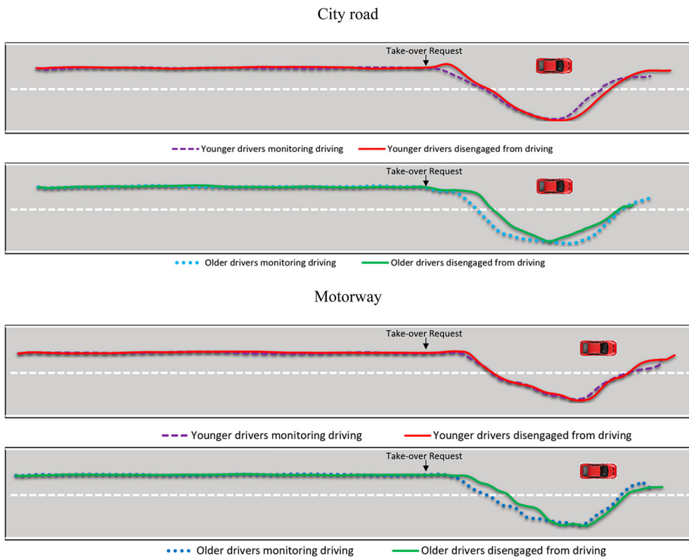
Figure 6. Average trajectories of participants' takeover control from the HAV on city road (top) and on motorway (bottom).
