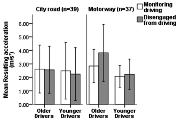
Figure 11. Resulting acceleration during takeover control process for different driver groups in different situations (error bars represent \pm 1 standard deviation of the mean).
