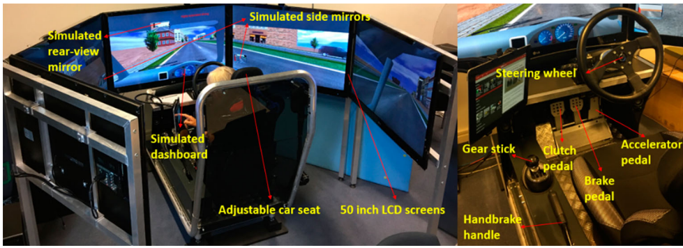
Figure 1. Fixed-based ST Software Jentig50 driving simulator.
