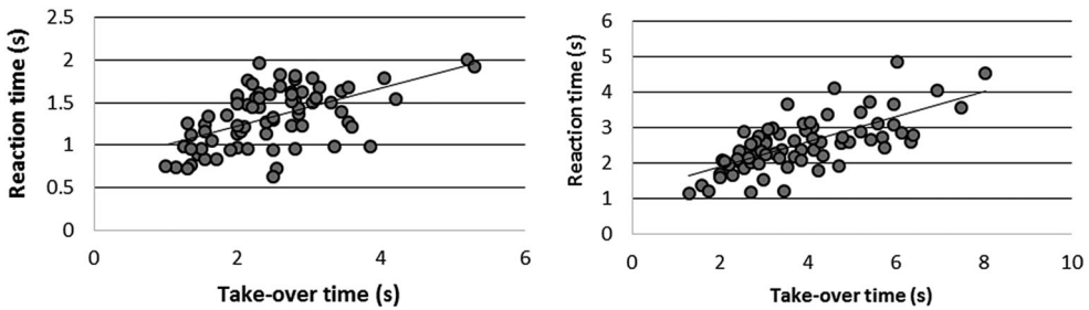
Figure 13. Correlation between the reaction time and takeover time of drivers when monitoring driving (left) and disengaged from driving (right).
