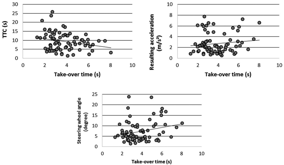
Figure 16. Correlation between the takeover time and takeover quality of drivers when disengaged from driving.
