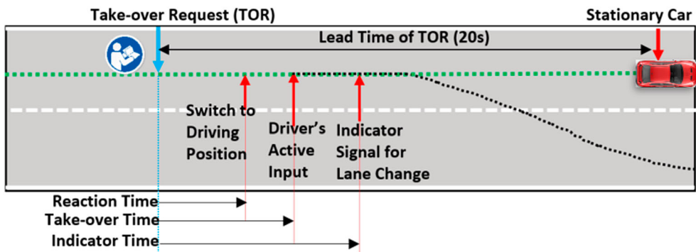
Figure 5. Time aspects of takeover.
