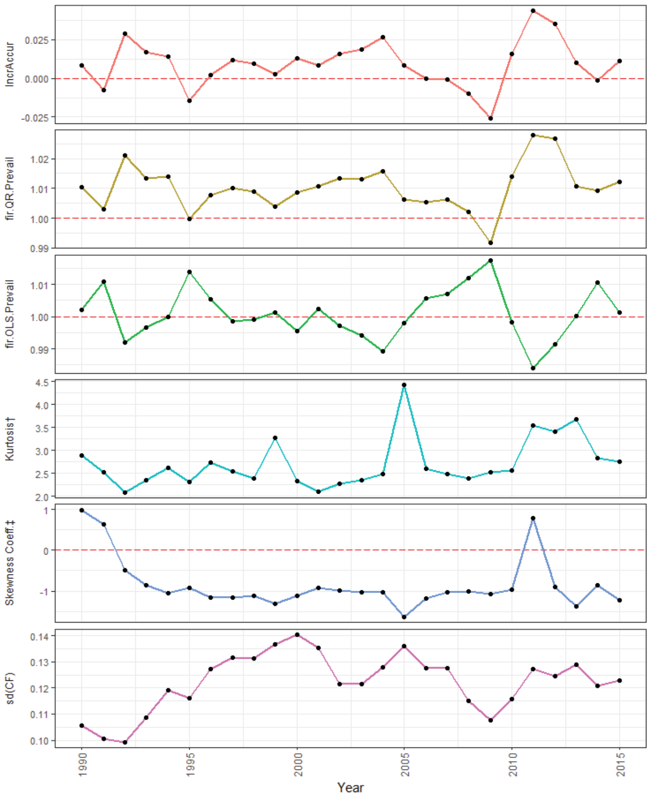
Figure 4. Incremental forecasting accuracy, forecast improvement ratios, and cash flows distributional properties: Quantile regression forecasting approach (versus OLS) for the first-order autoregressive cash flows model
