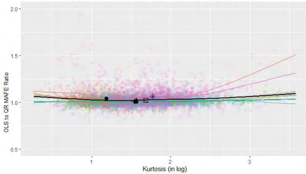
Figure 3a. Tail-Heaviness Effect on FIR of QR under MAFE
