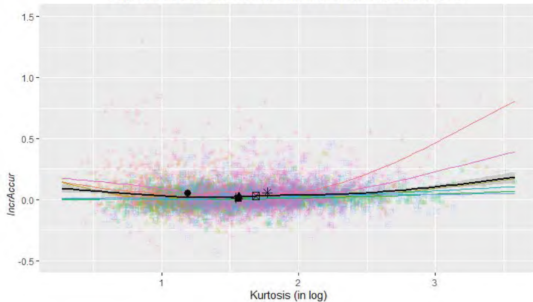
Figure 3c. Tail-Heaviness Effect on Incremental Accuracy of QR
