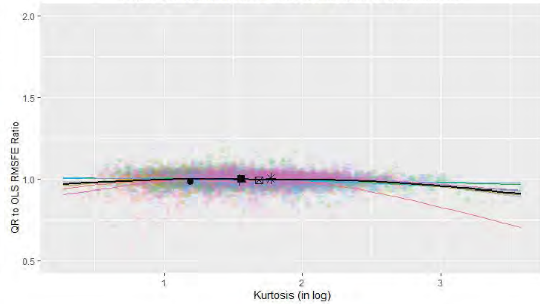
Figure 3b. Tail-Heaviness Effect on FIR of OLS under RMSFE
