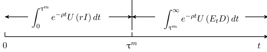
Figure 2: Irreversible investment under monopoly.
