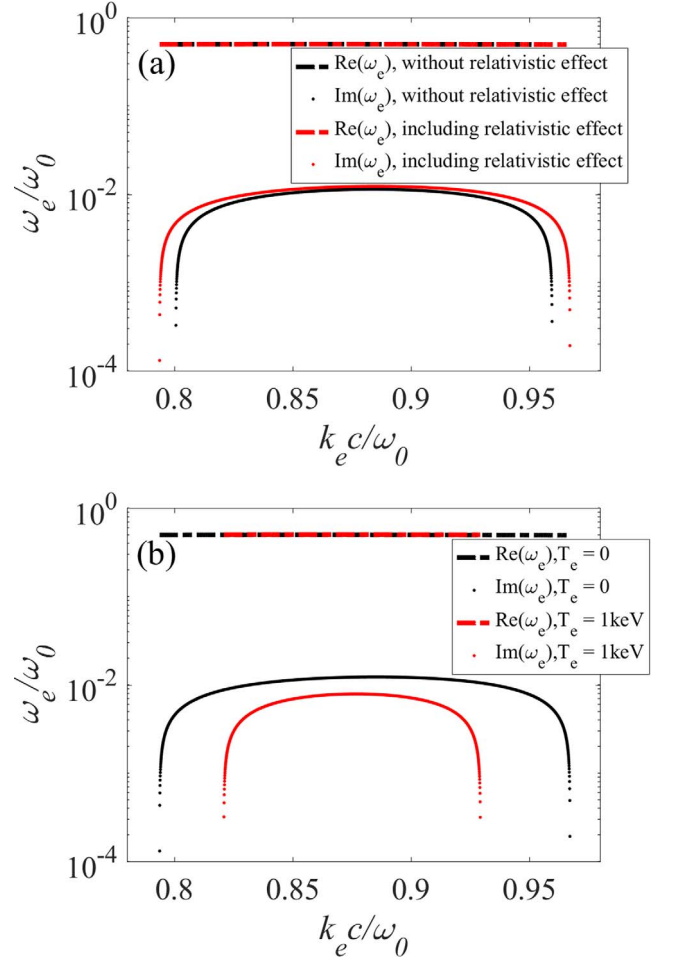
Figure 2. Numerical solutions of SRS dispersion equation at plasma density n_e = 0.27n_c with laser amplitude a_0 = 0.1 . (a) The relativistic modification on the non-eigenmode SRS at T_e = 0 . (b) The effect of electron temperature on non-eigenmode SRS. The dotted line and dashed line are the imaginary part and the real part of the solutions, respectively.
