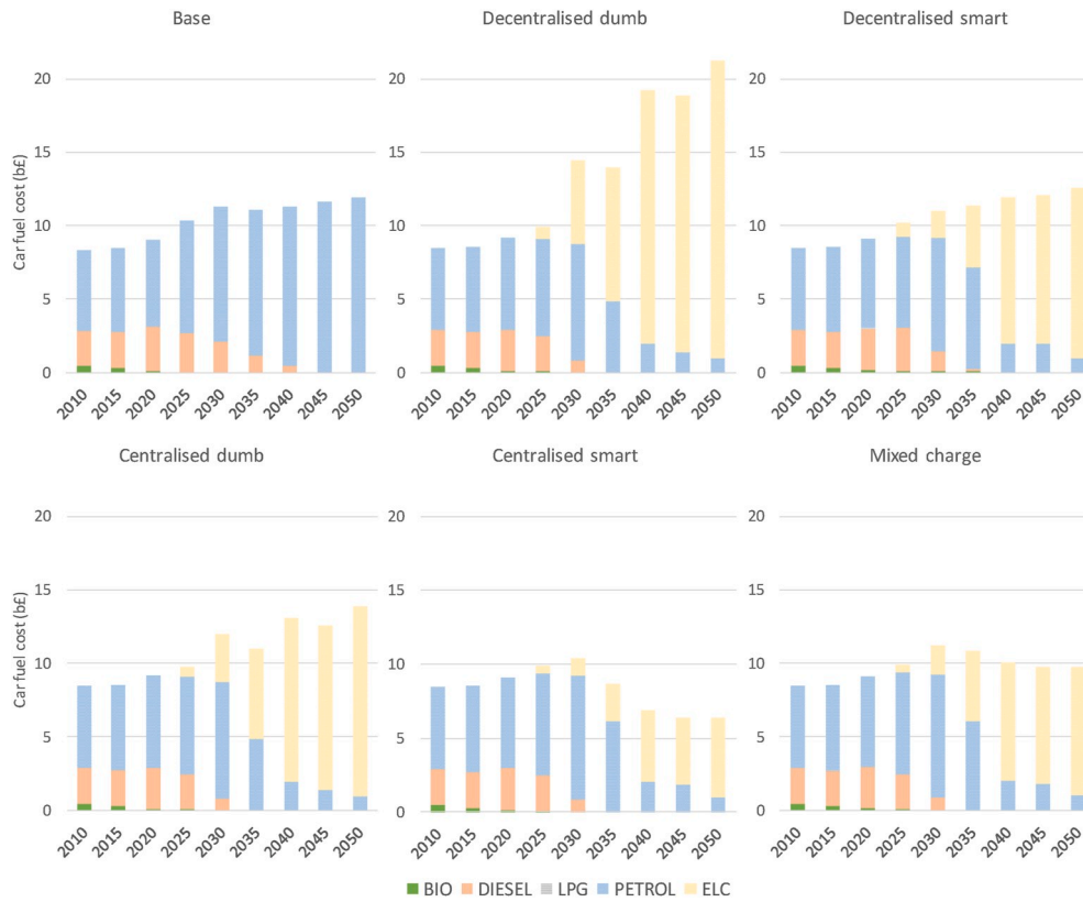
Fig. 8. Car transport energy cost per fuel type from year 2010–2050 for all EV charging scenarios.
