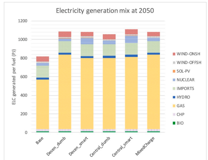
Fig. 10. Electricity generation per fuel type at 2050 for all scenarios.
