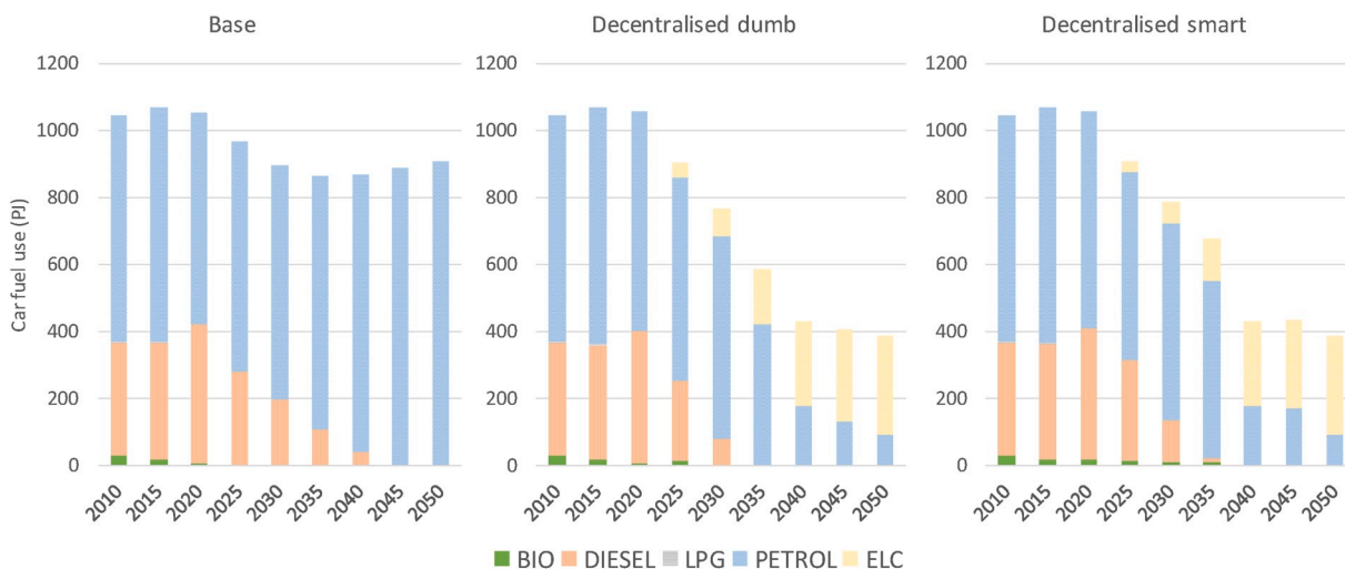
Fig. 7. Car transport energy use per fuel type from year 2010–2050 for the base, decentralised ‘dumb’ and decentralised ‘smart’ EV charging scenarios.
