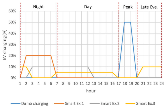
Fig. 4. EV demand profile examples for 'dumb' and 'smart' charging.
