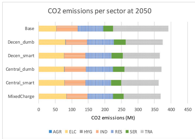
Fig. 9. CO 2 emission production per sector at 2050 for all scenarios.
