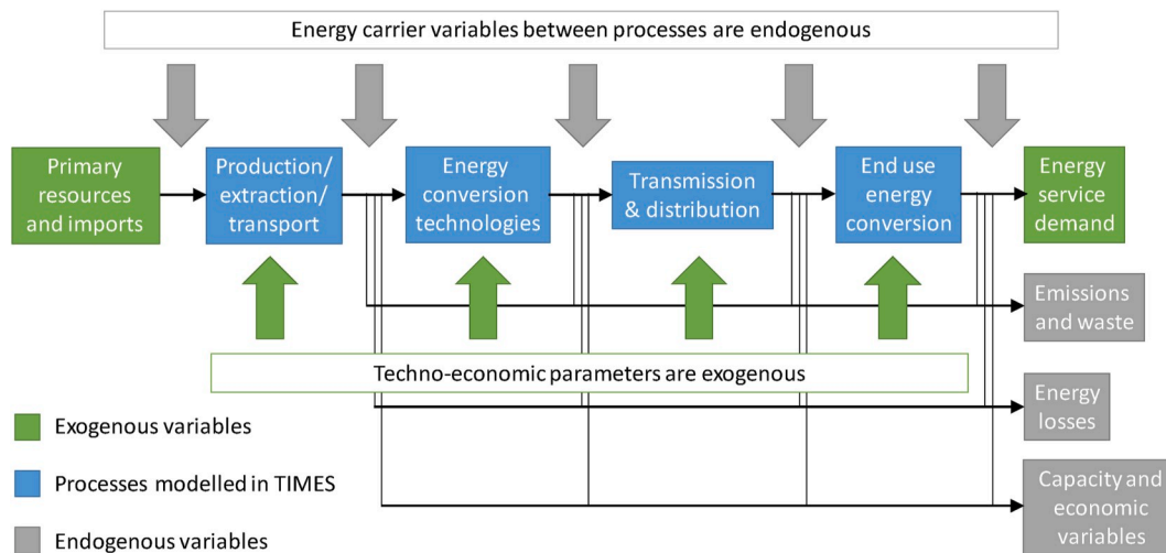
Fig. 1. Modelling of the energy system in TIMES (Calvillo et al., 2017).
