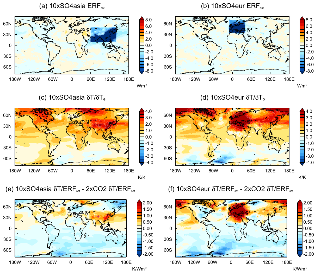
Figure 9. Multimodel mean ERF_{sst} for (a) 10xSO4asia and (b) 10xSO4eur. Multimodel mean surface temperature response normalized by the GSAT response for (c) 10xSO4asia and (d) 10xSO4eur. Multimodel mean difference in normalized surface temperature response relative to 2xCO2 for (e) 10xSO4asia and (f) 10xSO4eur. The temperature response is normalized by ERF_{sst} .
