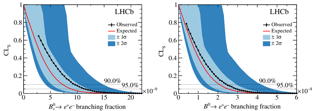
FIG. 2. \text{CL}_s values as a function of the branching fractions of the decays (left) B_s^0 \rightarrow e^+e^- and (right) B^0 \rightarrow e^+e^- . The red solid line (black solid line with data points) corresponds to the distribution of the expected (observed) upper limits, and the light blue (dark blue) band contains the 1\sigma ( 2\sigma ) uncertainties on the expected upper limits. Thresholds corresponding to 90% and 95% confidence level are indicated with dashed lines. The observed values are plotted for branching fractions greater than the measured branching fraction in the data; the test statistic is defined to be nonzero only in that region.
