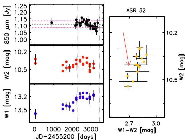
Figure 2. (Left-hand panels) WISE W1 (blue circles), W2 (red circles) magnitudes, and 850 \mu\text{m} flux from the JCMT for source 17 in NGC 1333. Horizontal lines are the same as in Fig 1. In the plots the black vertical dashed lines mark the time limits that were used to search for correlated variability between the WISE and JCMT data. (Right-hand panel) W2 versus W1 – W2 for the WISE data taken within the defined time limits. In the plot, the red arrow indicates the reddening vector with A_K = 0.5 mag, adapted from Indebetouw et al. (2005).
