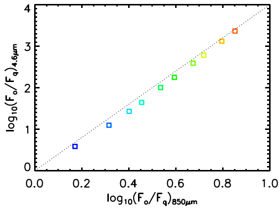
Figure 9. (Top panel) SED models of EC53 that result from increasing the protostellar luminosity by a factor 3.3–1000 from the fiducial model of the system. (Bottom panel) \log(F/F_0) ( WISE ) versus \log(F/F_0) ( JCMT ) for the various models of increase in protostellar luminosity, and for a disc inclination of 30^\circ . In the plot, the dashed black line represents \eta = 4 .
