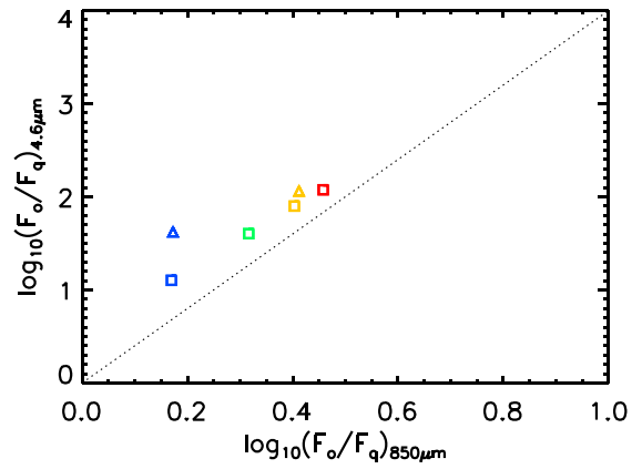
Figure 10. (Top panel) SEDs for the fiducial model of EC53 at 6 L_\odot (purple) and for increasing the luminosity to 20 (blue), 60 (green), 120 (orange), and 180 L_\odot (red). (Bottom panel) \log(F/F_0) ( WISE ) versus \log(F/F_0) ( JCMT ) for the different values of the luminosity. For each model, we tested using different radii for the boundary of viscous heating. For the 20 L_\odot radii of 1 au (blue square) and 3 au (blue triangle) are tested. For the 60 L_\odot , we set the boundary at 2.5 au (green square). Radii of 4 (orange square) and 10 au (orange triangle) are tested in the 120 L_\odot model. Finally, a radius of 6 au is used for the 180 L_\odot model.
