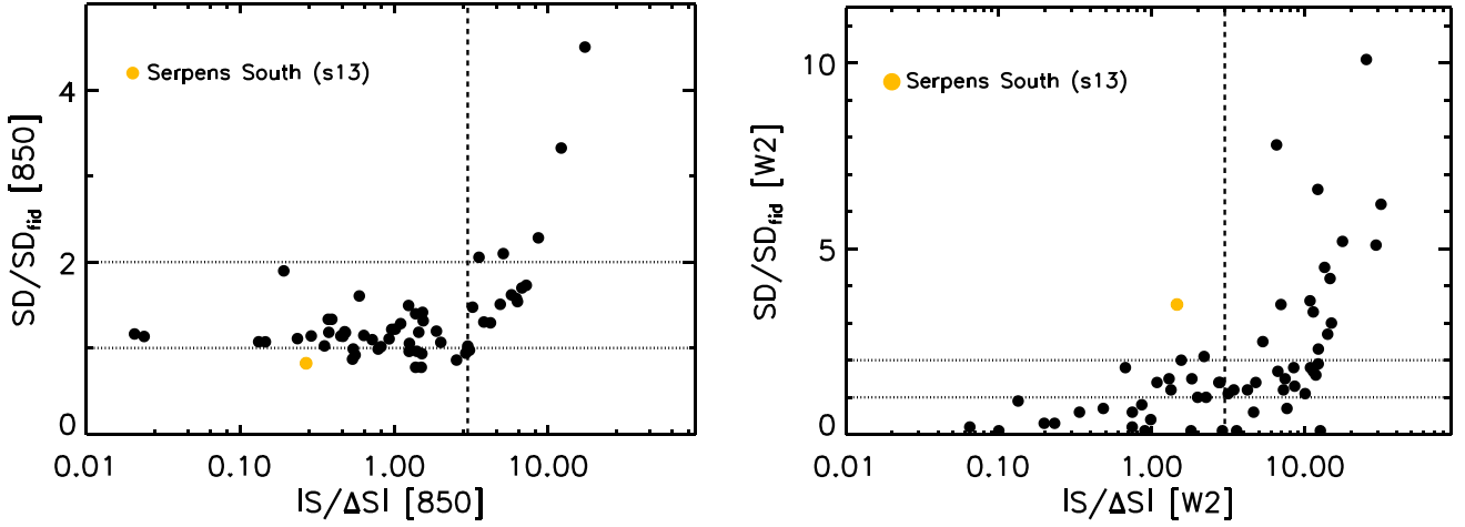
Figure 3. SD/SD_{fid} versus |S/\Delta S| for JCMT (left-hand panel) and WISE W2 (right-hand panel) data. In the plots, horizontal dotted lines mark the levels of SD/SD_{fid} equal to unity and SD/SD_{fid} = 2 . Objects found above the latter level are found to be stochastically variable objects. The vertical dashed lines mark |S/\Delta S| = 3 . Objects to the right-hand side of this line are candidates to display secular variability. The location of source 13 in Serpens South (see main text) is indicated by the orange solid circle. This object is discussed in more detail in Appendix B1.
