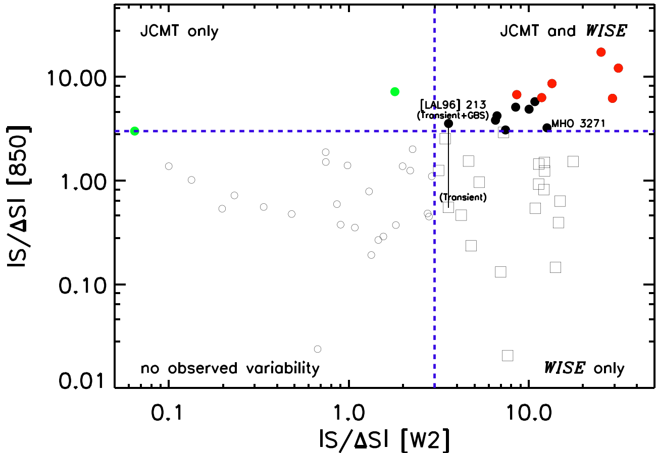
Figure 5. |S/\Delta S| (JCMT) versus |S/\Delta S| ( WISE W2) for the 59 targets in our sample. The blue dotted lines mark |S/\Delta S| = 3 , objects with values larger than this limit are strong variable candidates in both surveys. Depending on where objects locate, we can define 4 regions of variability. In the bottom left-hand quadrant, we find non-variable objects (open circles), the upper left-hand quadrant shows objects with variability only in the JCMT Transient Survey (green circles), while the bottom right-hand quadrant defines the region where we only observe variability at W2 (open squares). Finally, objects that are found to be variable in both surveys are located in the upper right-hand quadrant (solid circles). In the latter region, objects with the largest variability in both surveys |S/\Delta S| \geq 6 are marked by the solid red circles. In the figure, we mark the location of YSO [LAL96] 213, an object that moves between different regions when using additional data arising from the JCMT GBS (see Section 5), and YSO MHO 3271, an object that shows uncorrelated secular variability.
