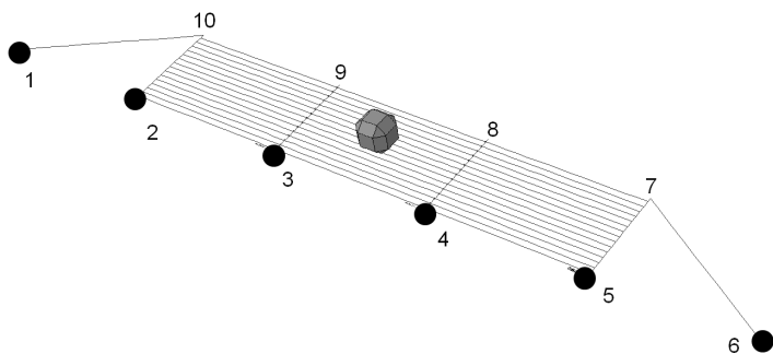
Figure 7. Three functional modules FE model of the ANAS barrier.
